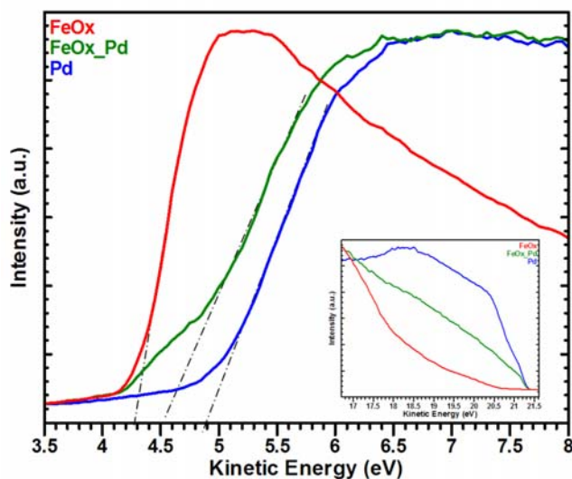
Figure 5. HeI spectra of secondary electron cutoffs for Fe@FeO x , Fe@FeO x /Pd and Pd NPs, the inset displays the Fermi energy region for all three NPs.
