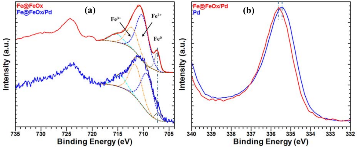
Figure 3. XPS spectra of (a) Fe 2p for Fe@FeO x and Fe@FeO x /Pd NPs and (b) Pd 3d for homemade Pd and Fe@FeO x /Pd NPs.
