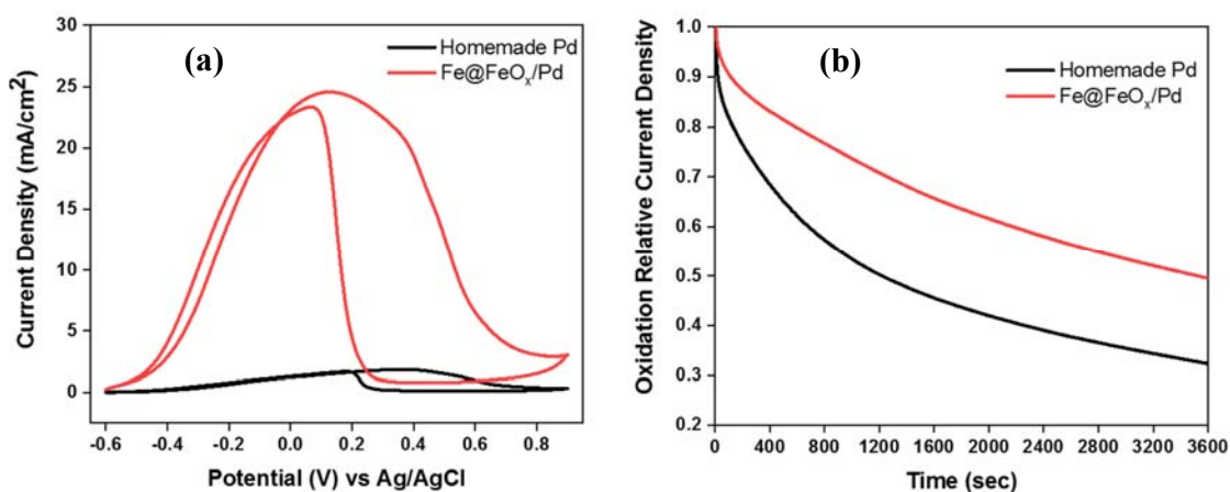
Figure 7. (a) Room-temperature CV results for Fe@FeO x /Pd and Pd NPs in 0.5 M KHCO 3 + 0.25M HCOOK at a scan rate of 20 mV/s under N 2 atmosphere, and (b) CA measurements at a fixed potential of 0.12 V of the same nanoparticles in the same electrolyte.
