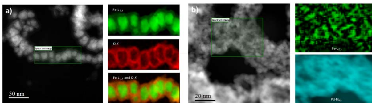
Figure 2. HRTEM images and their associated chemical mappings showing a) the core-shell structure of the Fe@FeO x NPs and b) the distribution of Pd (blue) covering the Fe@FeO x NPs (green).
