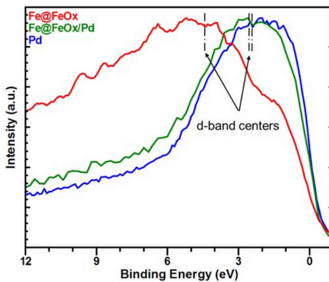
Figure 4. XPS valence band spectra for Fe@FeO x , Fe@FeO x /Pd, and homemade Pd NPs.
