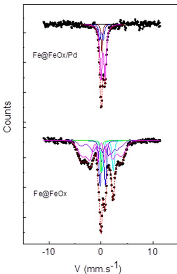
Figure 6. Mössbauer spectra for the Fe@FeO x and Fe@FeO x /Pd NPs obtained at room temperature.
