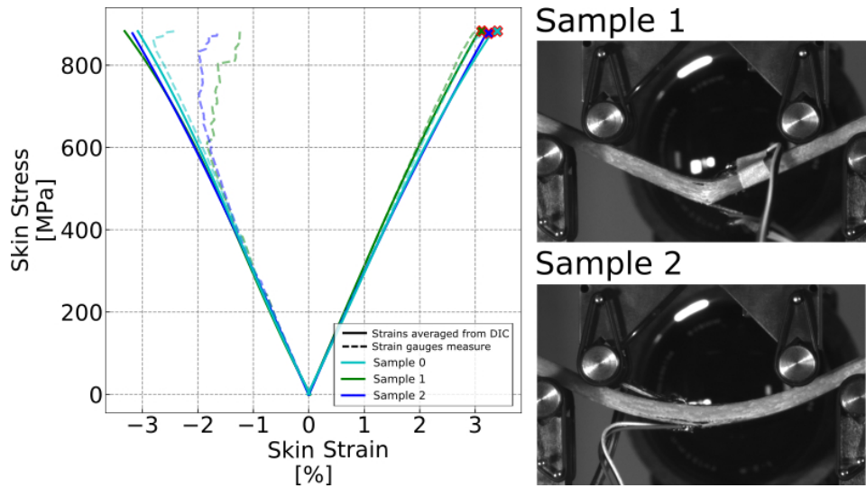
Figure 12: Four-point bending test: skin stress/strain results for three different E-glass/Epoxy specimens (cross = failure) and picture of the specimens just after collapse
