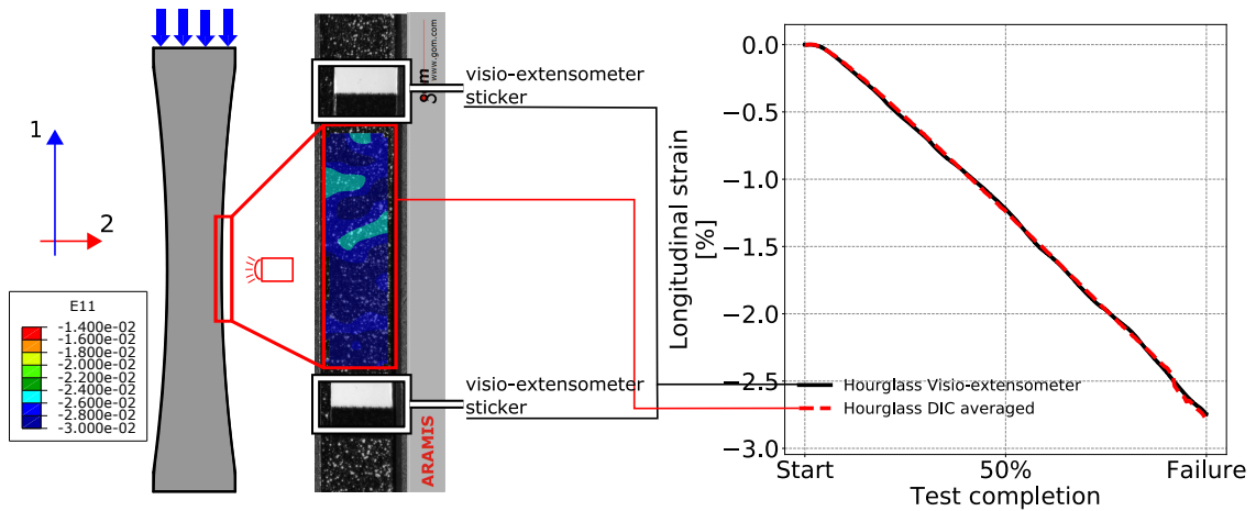
DIC longitudinal strain before failure Hourglass sample
