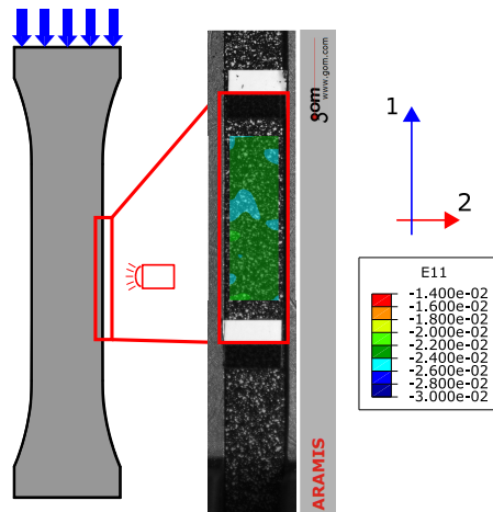
DIC longitudinal strain before failure Dog-bone sample
