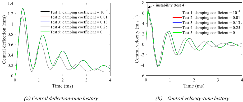
Fig. B1. Sensitivity studies regarding numerical damping (Rayleigh stiffness damping coefficients) on LS-DYNA/USA (DAA 1 ) results (Tests performed on carbon fiber/epoxy plate using P_0 = 1.5 MPa and \tau = 1.3 ms)
