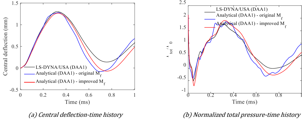
Fig. 6. Comparison between original and improved formulations of water-added mass (using CFRP plate subjected to an exponential loading of P_0 = 1.5 MPa and \tau = 1.3 ms)
