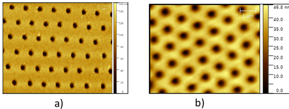
Fig. 10. AFM images on the square glass substrate of (a) S1805 photoresist layer structured by colloidal lithography and (b) gratings after deposition of absorbing multilayers.
