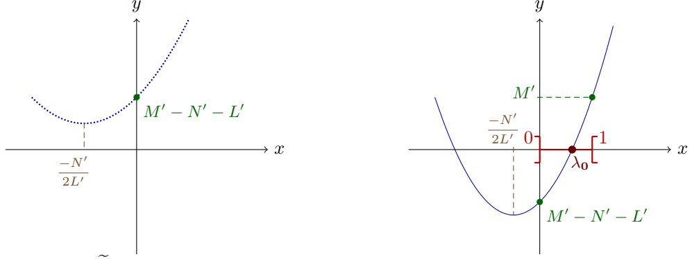
Figure 11: Polynomial \tilde{Q} for two set of parameters: the dotted line (.....) is associated with the case \mathbf{M}' - \mathbf{N}' - \mathbf{L}' > \mathbf{0} , the solid line (—) is associated with the case \mathbf{M}' - \mathbf{N}' - \mathbf{L}' < \mathbf{0} .
