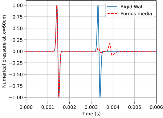
Figure 7: Numerical pressure signal over time at (x,y) = (0.6,0.1) , position of Mic. 2 in Fig. 6.
