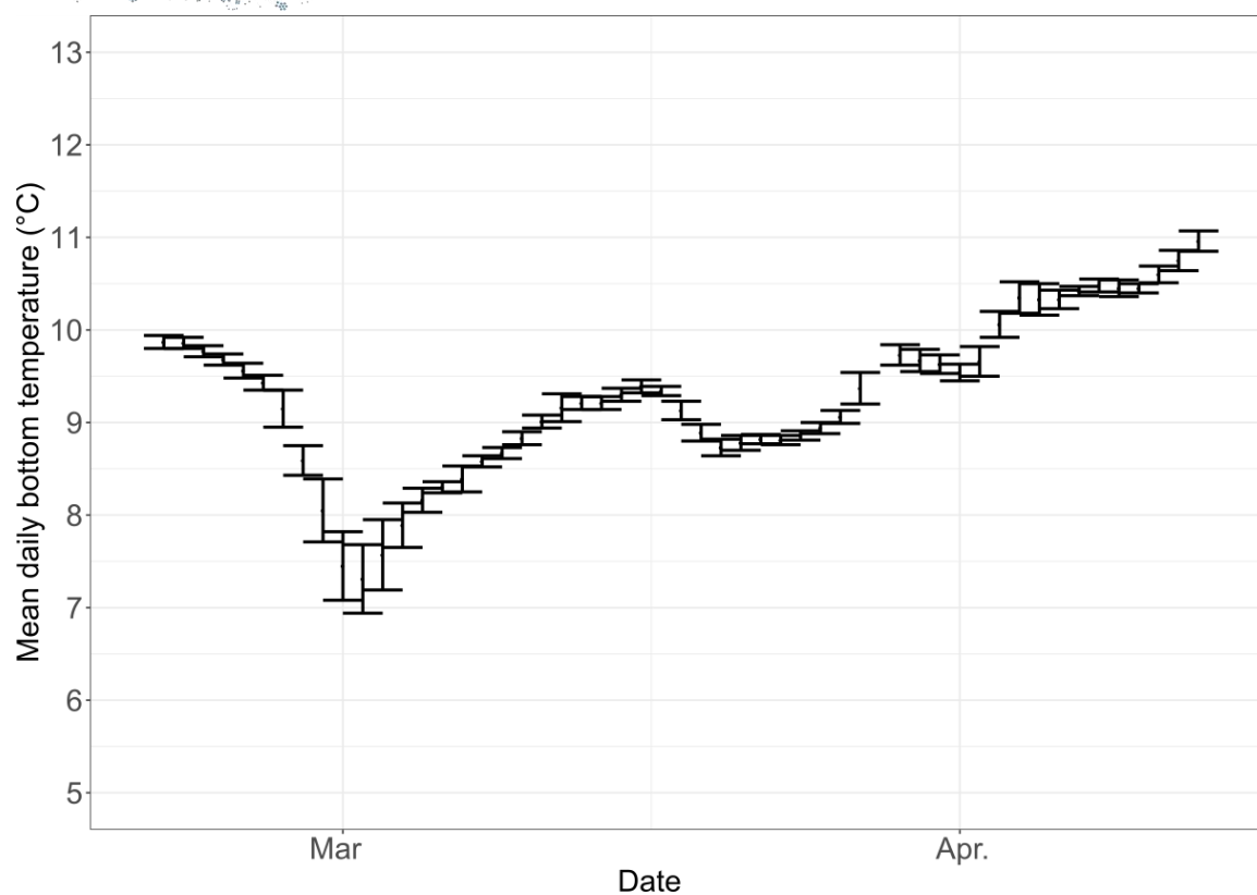
Figure S1: Mean daily temperature ( \pm SD) at the bottom in our study site.
