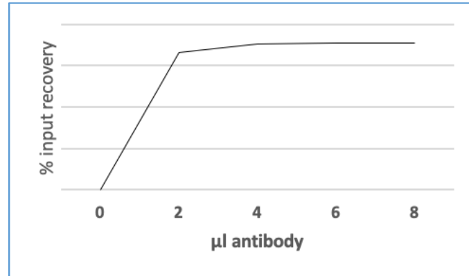
Figure 1. Schematic representation of a titration experiment where antibody saturation was reached at around 4 µl antibody.
