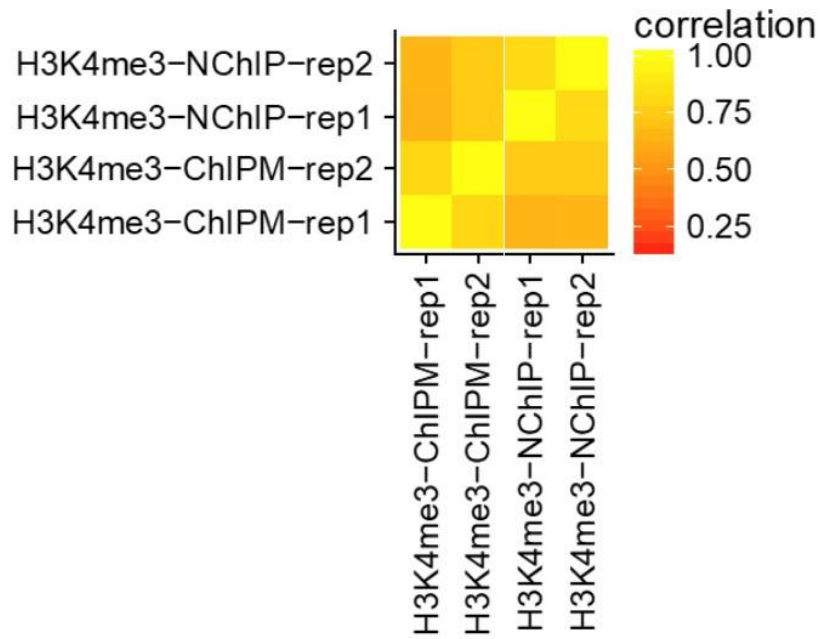
Figure 1. Heatmap of both nChIP and ChIPmentation for H3K4me3 representing similarity of 396 genome wide profiles and peak positions.
