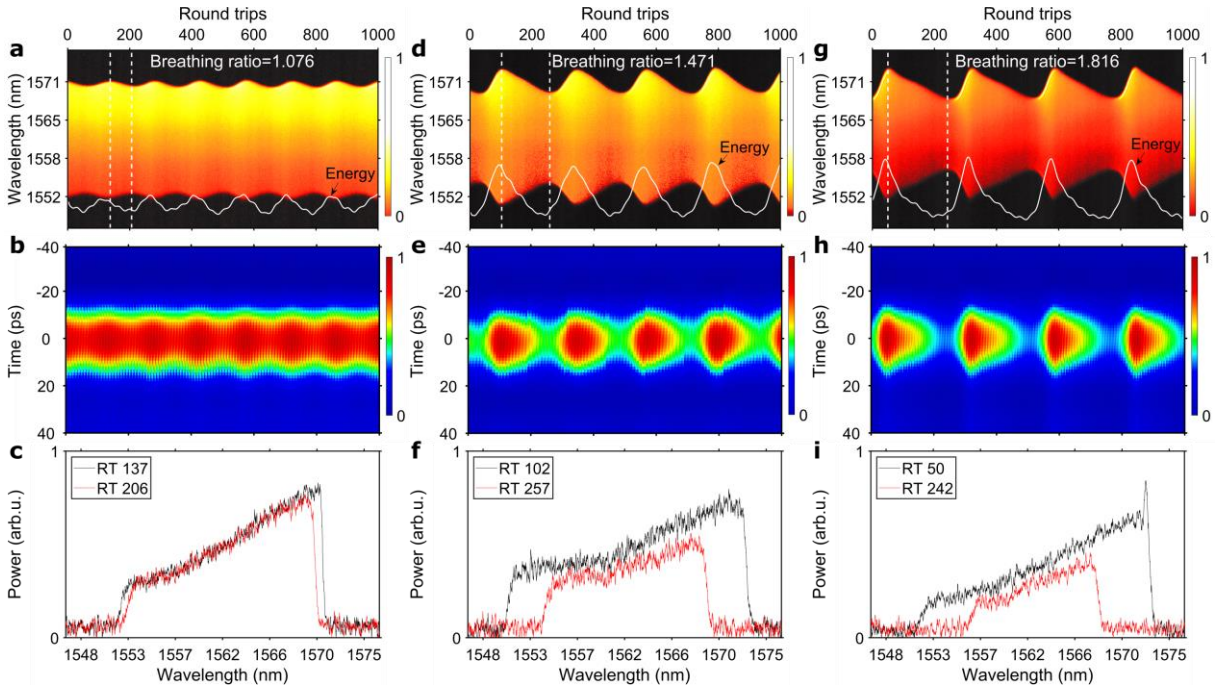
Fig. 3 EA optimisation results for breathing solitons with a tunable breathing ratio: dynamics of breathers with (a-c) small, (d-f) moderate and (g-i) large breathing ratios. (a,d,g): DFT recording of single-shot spectra over consecutive cavity round trips. (b,e,h): Temporal evolution of the intensity relative to the average round-trip time over consecutive round trips. (c,f,i): Single-shot spectra at the round-trip (RT) numbers of maximal and minimal spectrum extents within a period.
