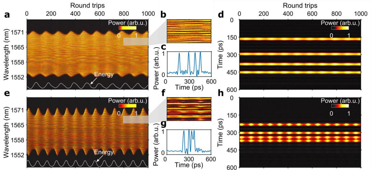
Fig. 7 Typical EA optimisation results for BMCs formed of four breathers: Dynamics of (1+3) BMCs with (a-d) large and (e-h) small internal pulse separations. (a,e) DFT recording of single-shot spectra over consecutive cavity round trips. The white curve represents the energy evolution. (b,f) Close-up view of the DFT recording. (c,g) Corresponding temporal intensity. (d,h) Temporal evolution of the intensity relative to the average round-trip time over consecutive round trips.
