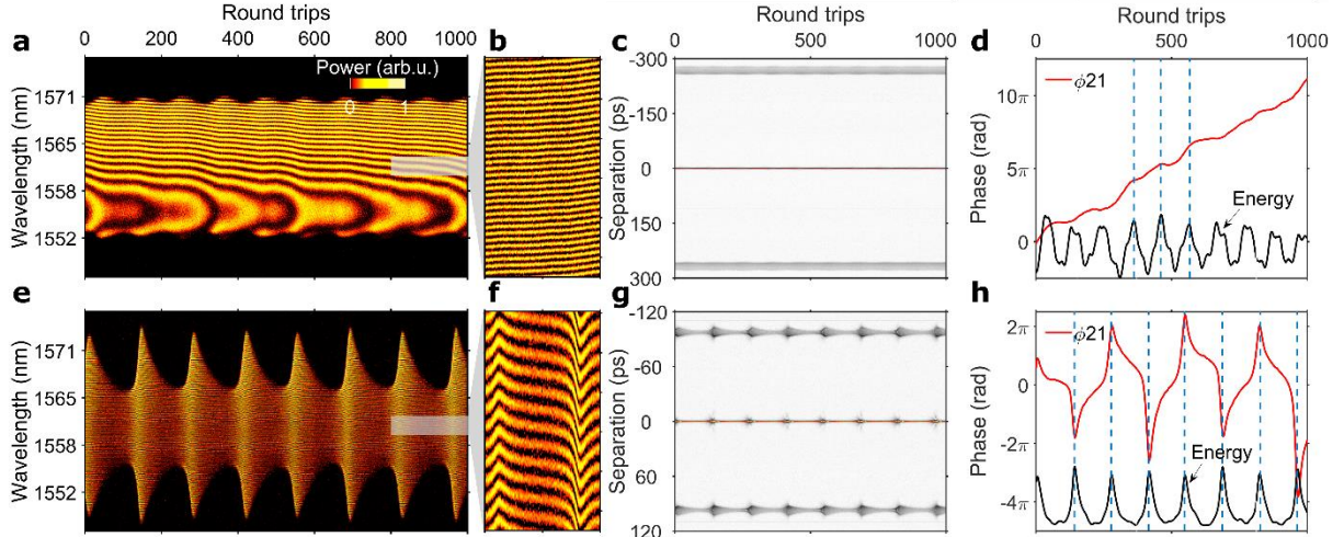
Fig. 5 Typical EA optimisation results for breather-pair molecules: Dynamics of (a-d) “increasing-phase” and (e-h) “oscillating-phase” breather molecules. (a,e) DFT recording of single-shot spectra over consecutive cavity round trips. A Moiré interference pattern is visible in panel (a). (b,f) Close-up view of the DFT recording. (c,g) Evolution of the first-order single-shot autocorrelation trace over consecutive round trips. (d,h) Evolution of the phase difference between the two breathers (red curve) and the energy of the molecule (black curve) as a function of the RT number.
