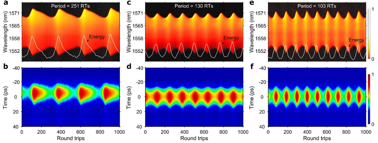
Fig. 4 EA optimisation results for breathing solitons with a tunable oscillation period: Dynamics of breathers with (a-b) large, (c-d) moderate and (e-f) small oscillation periods. (a,c,e): DFT recording of single-shot spectra over consecutive round trips. The white curve represents the energy evolution. (b,d,f): Temporal evolution of the intensity relative to the average round-trip time over consecutive round trips.
