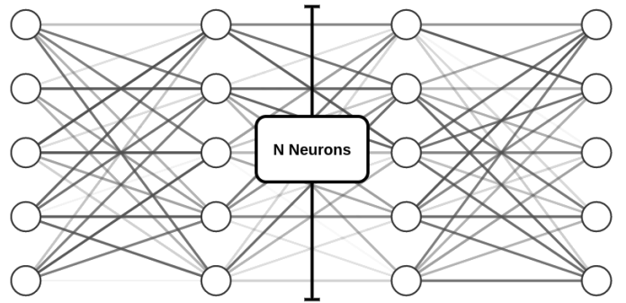
FIGURE 1 The proposed architecture is composed of 4 fully connected layers of size the number of dofs with a PReLU activation function.
