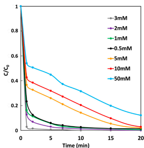
Figure 9. Effect of H 2 O 2 concentration on the degradation of MG dye during the GF process.
