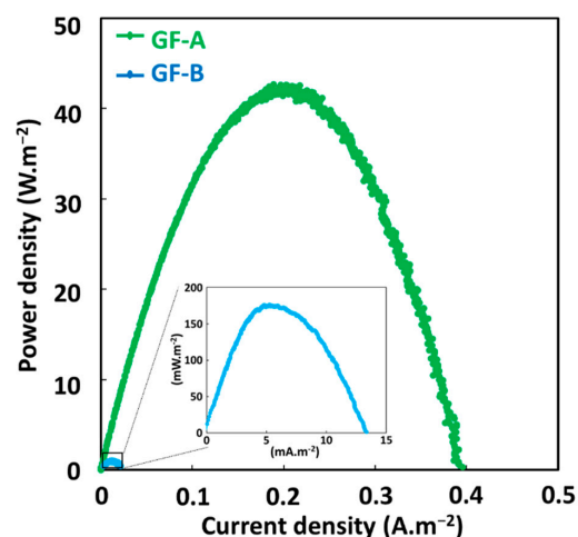
Figure 5. Power curves of the GF process obtained under GF-A (green line) and GF-B (blue line) conditions.
