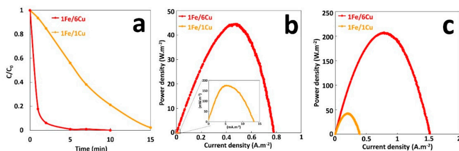
Figure 6. (a) Effect of Cu/Fe area ratio on the degradation of MG dye during the GF process, (b) Power curves of the GF process obtained with different Cu/Fe area ratios during degradation process (GF-B configuration), (c) Power curves of Fe/Cu couple without the Fenton reaction for different area ratios (GF-A configuration).
