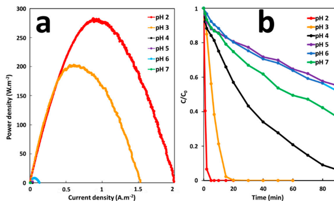
Figure 7. (a) Power curves of the GF process obtained at different pH and (b) Effect of pH on the degradation of MG dye during the GF process.
