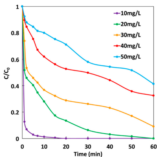
Figure 10. Effect of MG concentration on the degradation rate during the GF process.
