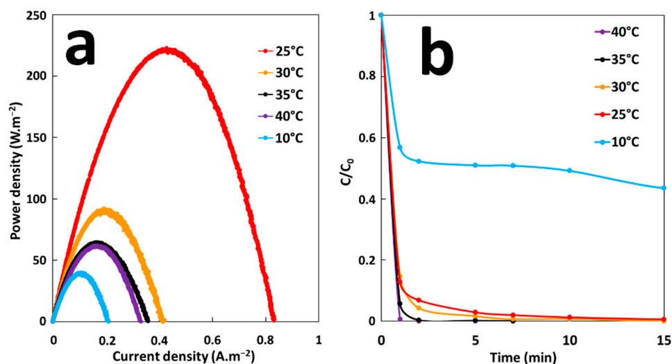
Figure 8. (a) Power curves of the GF process obtained at different temperatures and (b) Effect of temperature on the degradation of MG dye during the GF process.
