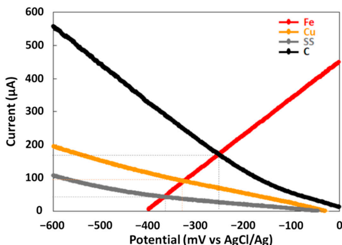
Figure 3. Corrosion potential and current corrosion of iron electrode coupled to different cathodes.
