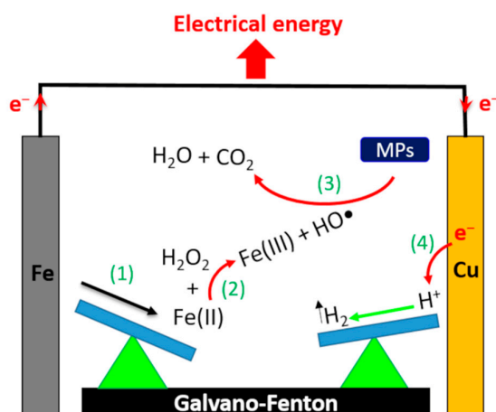
Figure 1. Schematic representation of the mechanism for producing electrical energy with the Galvano-Fenton process.
