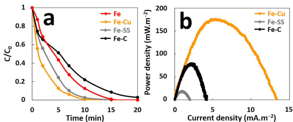
Figure 2. (a) Effect of cathode material on the decolorization of MG dye during the GF process, (b) Power curves of the GF process obtained with different cathode materials.
