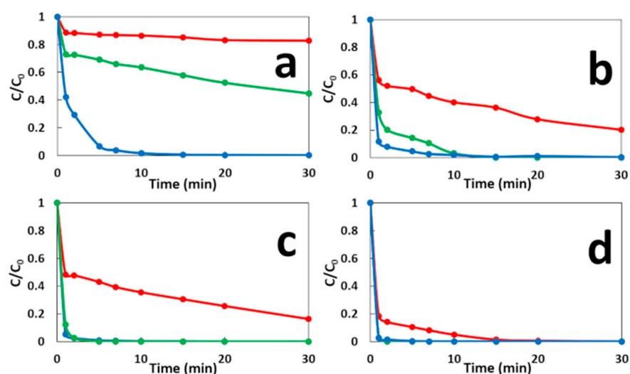
Figure 4. Effect of the cathode material on the decolorization of MG dye during the GF-A process (green line) and the GF-B process (blue line) for: (a) 2.7 \text{mg}\cdot\text{L}^{-1} of \text{Fe}^{2+} /1 min immersion, (b) 8 \text{mg}\cdot\text{L}^{-1} of \text{Fe}^{2+} /5 min immersion, (c) 11.8 \text{mg}\cdot\text{L}^{-1} of \text{Fe}^{2+} /10 min immersion, and (d) 17.8 \text{mg}\cdot\text{L}^{-1} of \text{Fe}^{2+} /20 min immersion. The CF process (red line) is presented for comparison.
