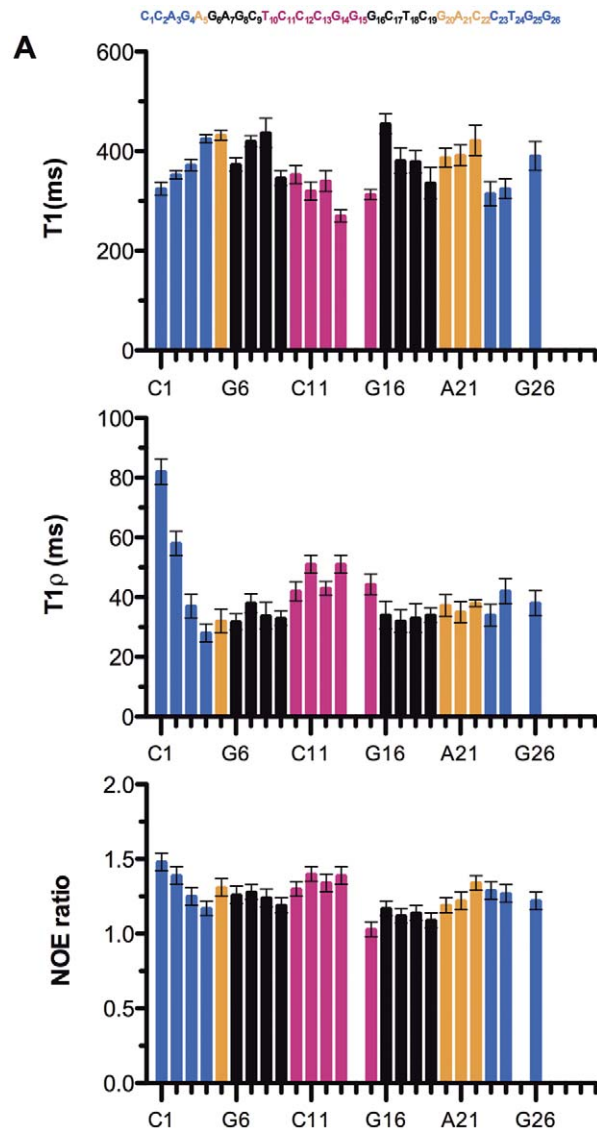
Figure 3. Relaxation times for aromatic C6/C8 spins of mini-cTAR DNA at 500 MHz. Top to bottom: ^{13} C T_1 , ^{13} C T_{1\rho} and hetNOEs. Errors represent uncertainties in the fit of the primary relaxation data to mono-exponential decays. No data are associated to residues corresponding to a broad or overlapped cross peak. The color codes used for the residues are the following: blue (lower stem), orange (internal loop), black (upper stem) and magenta (apical loop). doi:10.1371/journal.pone.0038905.g003
