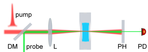
FIG. 4. Experimental setup of ns TL spectroscopy: DM, dichroic mirror; L, lens; PH, pinhole; and PD, photodetector.
