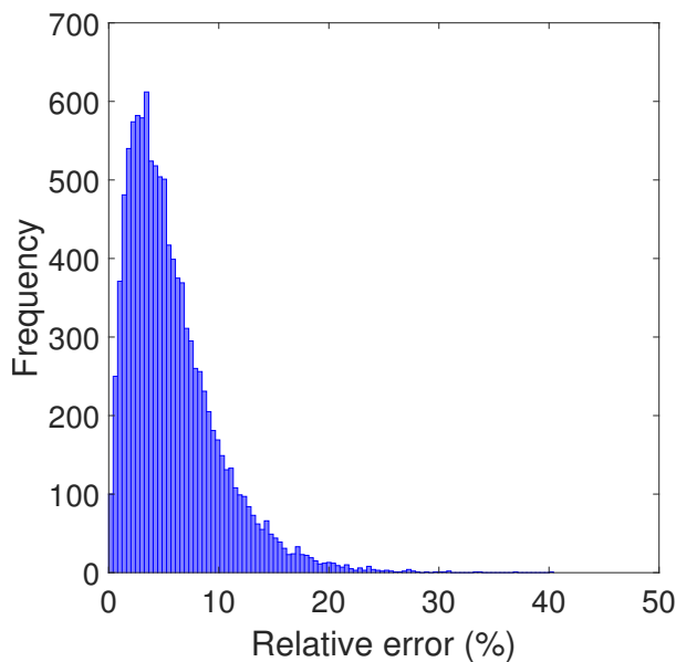
Fig. 3.2: Histogram of the relative deviation of the bound given in Lemma 2 for all 11,117 connected graphs with 8 nodes.
