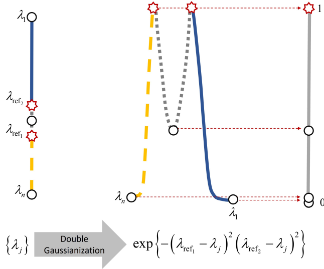
Fig. 9.2: Schematic illustration of the double Gaussianization of the graph spectra. The eigenvalues of the adjacency matrix are folded at two different reference eigenvalues and then exponentiated as illustrated in the right part of the figure.
