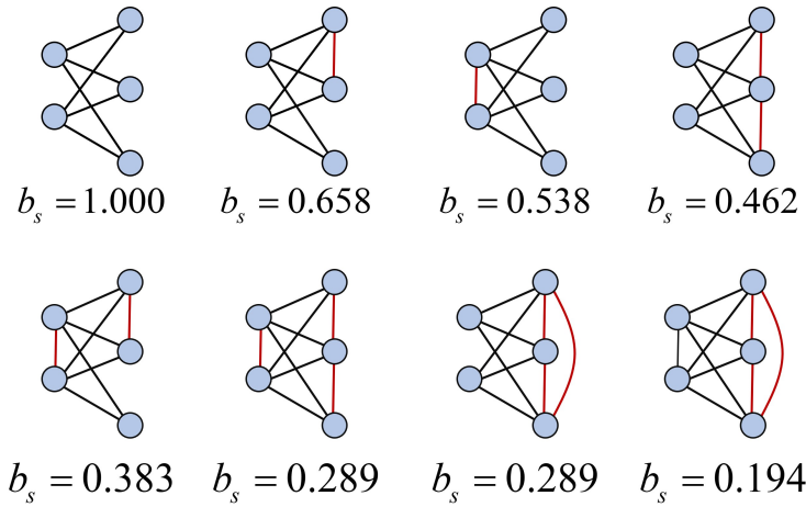
Fig. 8.1: Illustration of the change in the bipartivity index with the increase in the number of edges in a complete bipartite graph.
