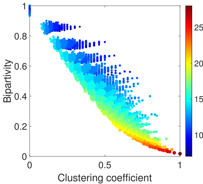
Fig. 8.3: Scatter plot of the bipartivity and the clustering coefficient of all connected graphs with 8 nodes. The points in the plot are colored by the number of edges that the corresponding graph has.
