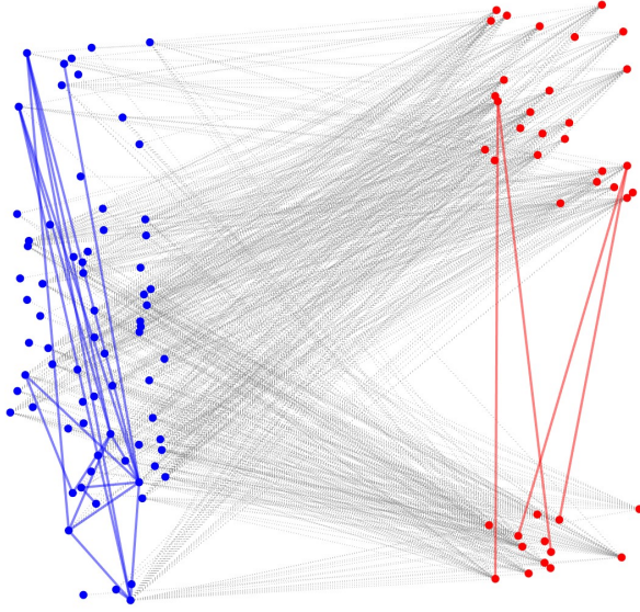
Fig. 8.4: Illustration of a bipartition of the network of Stony stream using the method developed by [82]. The dotted lines joints the two partitions and continuous lines connect vertices inside the same partition, i.e., they frustrate the bipartition of the network.
