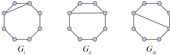
Fig. 10.1: Examples of three graphs with 8 nodes and chordless cycles of different lengths: G_I has a triangle and an heptagon; G_{II} has a square and a hexagon; G_{III} has two pentagons.
