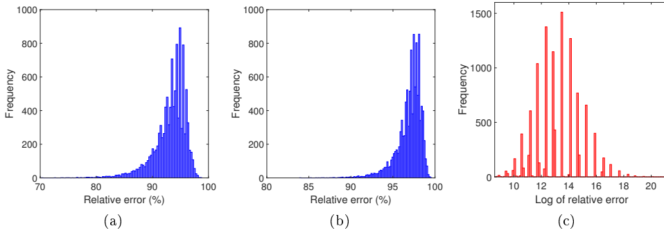
Fig. 14.1: Histogram of the relative deviations for the lower bounds Theorem 37 and Theorem 38 (in %) as well as of the upper bound Theorem 37 (as logarithm) for all 11,117 connected graphs with 8 nodes.
