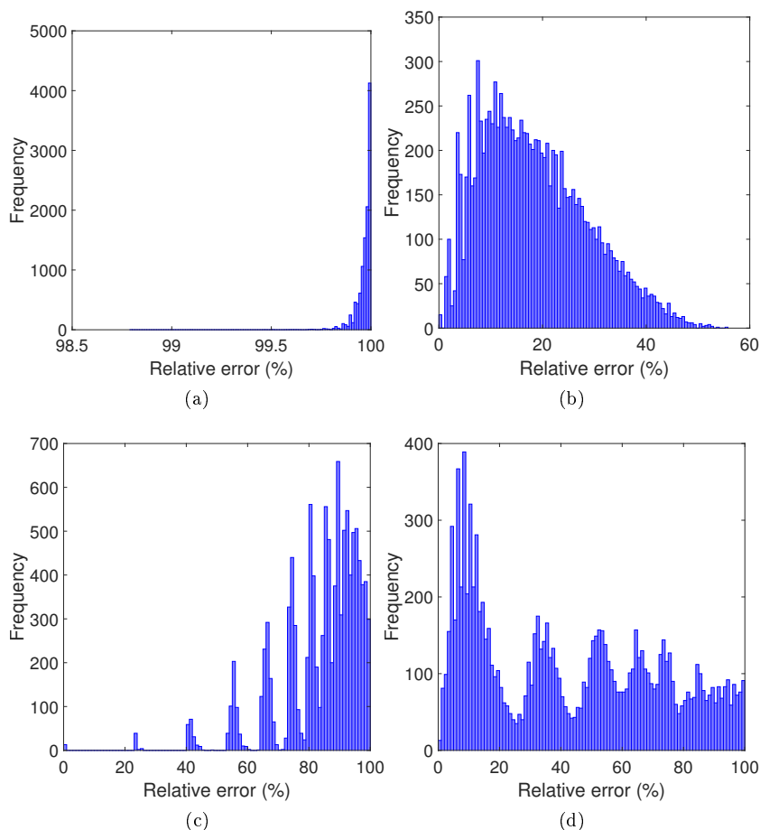
Fig. 16.3: Relative deviations of the lower bounds in Theorem 44, Theorem 45, Theorem 46 and Theorem 47 for all connected graphs with 8 nodes.
