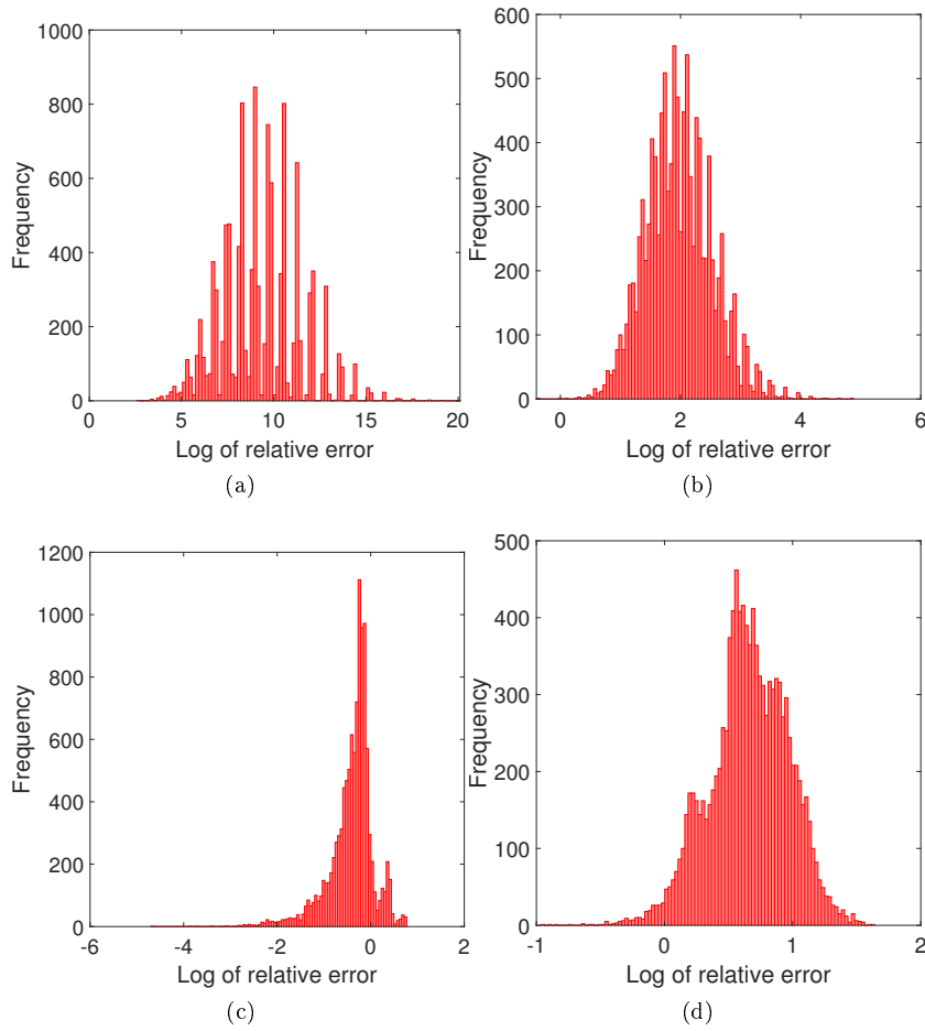
Fig. 15.2: Relative deviation (in logarithmic scale) of the upper bounds given in Proposition 2, Proposition 3, Theorem 41 and Theorem 42 for all connected graphs with 8 nodes.
