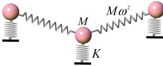
Fig. 11.1: Illustration of a system formed by three balls of mass M tied to the ground with springs of constant K connected by springs of constant M\omega^2 .
