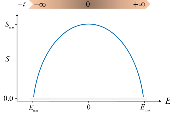
Fig. 8.2: Sketch of the plot of entropy versus energy used to illustrate the definition of the inverse temperature which is given by the slope of the curve in a given point. The scale of inverse temperature is given on top of this plot.
