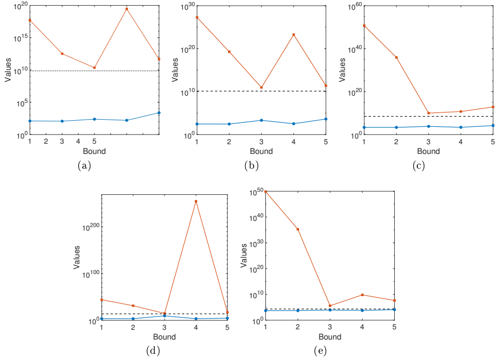
Fig. 5.2: Plot of the estimates of the lower (blue circles) and upper (red squares) for the bounds: (1) (Theorem 5), (2) (Theorem 6), (3) (Theorem 7 using a = -\lambda_1 and b = -\lambda_n ), (4) (Theorem 7 using a = -k_{max} and b = k_{max} ), (5) (Theorem 8). The results are for (a) Stony, (b) neurons, (c) yeast, (d) internet and (e) powergrid. The dashed lines represents the “exact” value of the Estrada index for the networks. Very large values are obtained by using variable-precision floating-point arithmetic (vpa) in Matlab.
