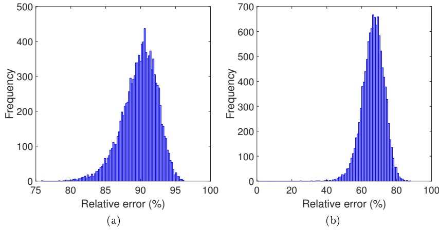
Fig. 9.3: Histograms of the relative deviations in percentage of the bounds given in Theorem 30 and in Theorem 32 for all connected graphs with 8 nodes.
