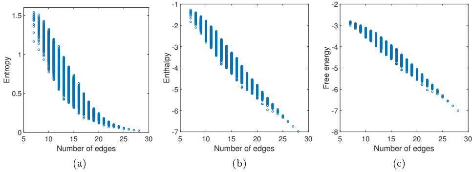
Fig. 6.1: Plots of the entropy (a), enthalpy (b) and free energy (c) versus the number of edges in all connected graphs with 8 nodes.
