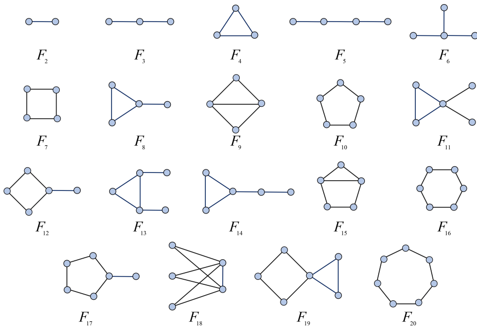
Fig. 3.1: Illustration of the small subgraphs appearing in the first seven spectral moments of the adjacency matrix of simple graphs.
