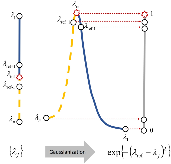
Fig. 9.1: Illustration of the gaussianized spectrum method. The eigenvalues of the adjacency matrix of the network are folded at \tilde{\lambda} into the spectrum of (\tilde{\lambda}I - A)^2 . Then they are exponentiated to give more weight to \lambda_{\text{ref}} .
