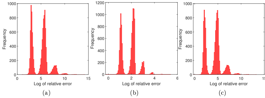
Fig. 16.4: Relative deviations (in logarithmic scale) of the upper bounds given in Theorem 44, Theorem 45 and Theorem 46 for all connected graphs with 8 nodes.
