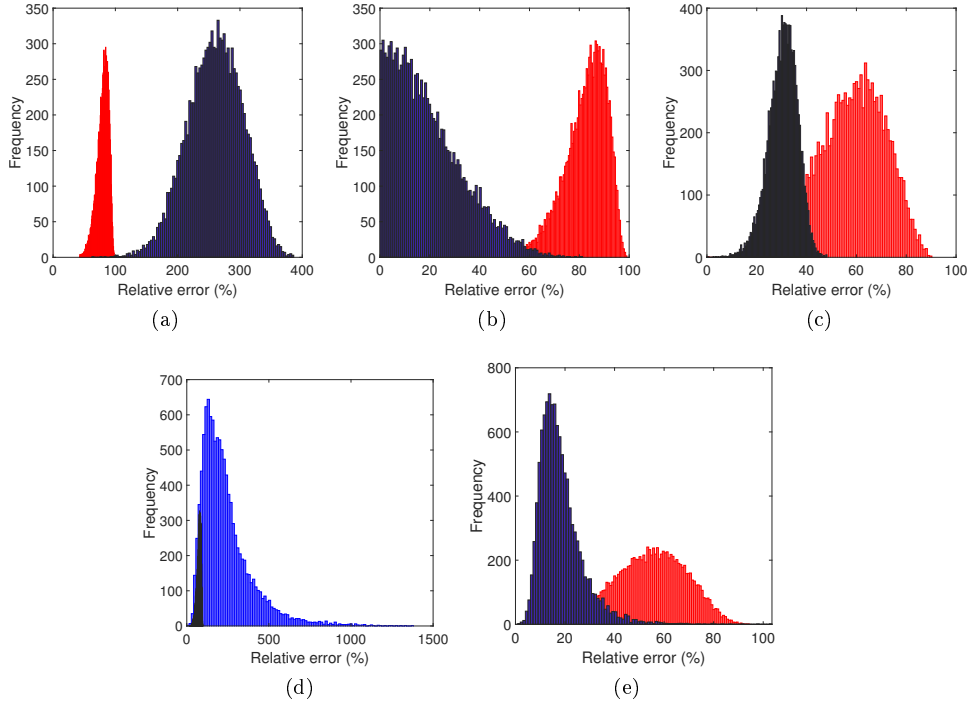
Fig. 5.1: Histograms of the relative deviations in percentage for: (a) Bound 1 (Theorem 5), (b) Bound 2 (Theorem 6), (c) Bound 3 (Theorem 7 using a = -\lambda_1 and b = -\lambda_n ), (d) Bound 4 (Theorem 7 using a = -k_{max} and b = k_{max} ), (e) Bound 5 (Theorem 8). In blue we illustrate the histogram for the lower and in red for the upper bounds. As usual for histograms, frequency stands for the number of graphs in each bin.
