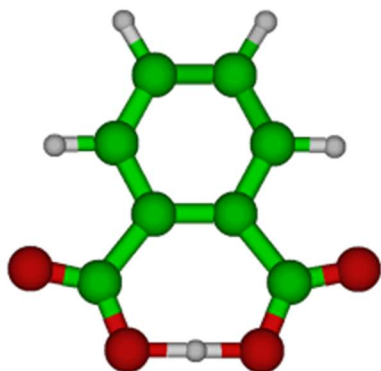
Figure 4. Calculated optimized structures of the deprotonated monoanion (left) and of the radical (right) at the aug-cc-pVDZ/CAM-B3Lyp level. The anion has a Zundel-type structure and thus a C_{2v} symmetry; in the radical the H is localized on one of the oxygen atoms. The Cartesian coordinates are given in the SI.
