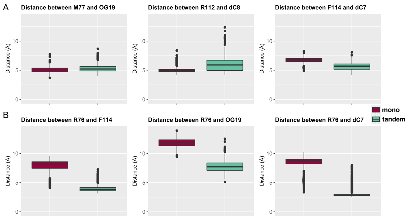
Figure 3. Distribution of relevant distances involving the intercalation triad (A) and R76 (B) upon a single 8-oxoG mutation (single) or Ap + 8-oxoG lesions (tandem). The presence of the Ap site at position 20 makes M77 and R112 move away from 8-oxoG and the facing dC8. Steric hindrance provoked by R76 movement pushes F114 closer to dC7. R76 comes closer to 8-oxoG and intercalates in the gap left by the abasic site, with formation of very stable H-bonds bridging Ap20 and the facing dC7. It also interacts with F114, preventing it to stack within the double-helix.
