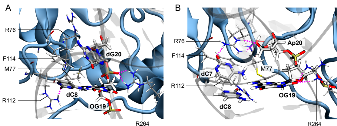
Figure 2. Cartoon representation of MutM interacting with the DNA helix harboring a single 8-oxoG lesion (OG19, A) or tandem lesion 8-oxoG + Ap (OG19 and Ap20, B). H-bonds are depicted as dashed pink lines and the DNA structure is rendered transparent for sake of clarity. Upon local multiple lesions, the interaction pattern around 8-oxoG (OG19) is perturbed. The intercalation triad M77/R112/F114 is shifted down by R76 which comes to interact between Ap20 and the facing dC7, preventing M77 and F114 intercalation above 8-oxoG. R264, normally interacting with the DNA backbone phosphates between positions 19 and 20, is now involved in hydrogen bonding with OG19 carbonyl.
