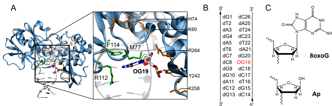
Figure 1. (A) Cartoon representation of the bacterial MutM in interaction with a 13-bp double stranded DNA helix harboring 8-oxoguanine (OG19) as the 19th nucleobase — PDB ID code 3GO8 27 . The magnified section highlights the position of the catalytic triad (M77, R112, and F114 in green) and the residues interacting with the DNA backbone (in orange) around the damage. (B) Sequence of the 13-bp oligonucleotide, showing the position of the 8-oxoguanine (in red). In simulations with tandem lesions, dG20 is mutated in silico into an abasic site (Ap). (C) Chemical structure of the 8-oxoguanine and the abasic site lesions.
