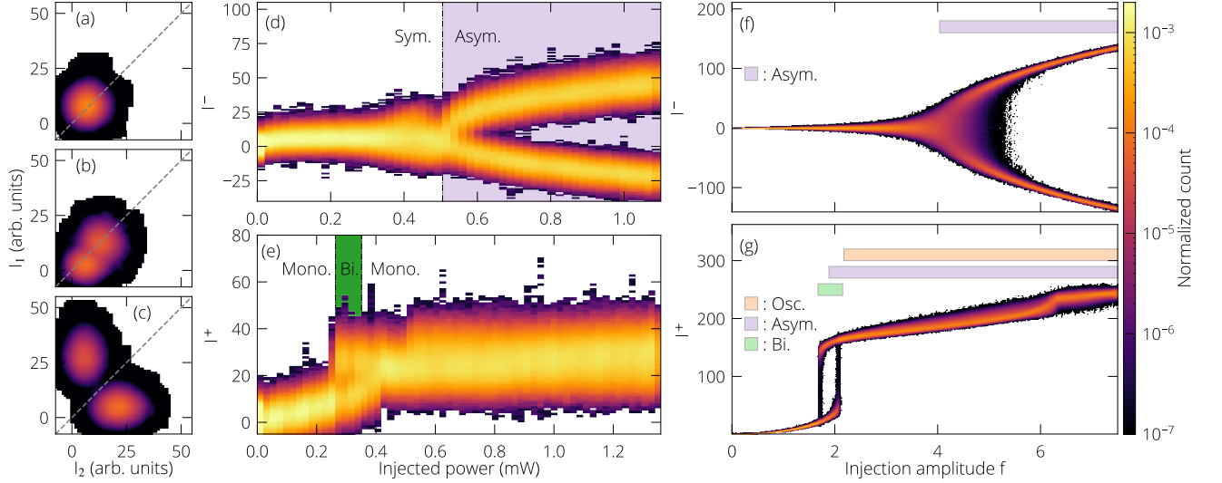
FIG. 4. Identification of operational regimes. (a)-(c) Selected projections of the phase space showing monostable symmetric, bistable symmetric, and bistable asymmetric steady states, respectively. (d), (e) Experimental and (f), (g) numerical histograms computed from 500 realizations, showing I^- [(d), (f)] and I^+ [(e), (g)] versus injection strength. (a) 0.22 mW. (b) 0.26 mW. (c) 1.03 mW. (a), (c) \delta = -0.82 . (d), (f) \delta = -2.86 . (b), (e), (g) \delta = -6.19 .
