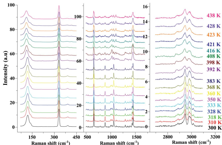
Fig. 6 Temperature evolution of the Raman spectra for selected spectral ranges [70 – 450 \text{ cm}^{-1}] , [500 – 1700 \text{ cm}^{-1}] and [2700 – 3200 \text{ cm}^{-1}] .
