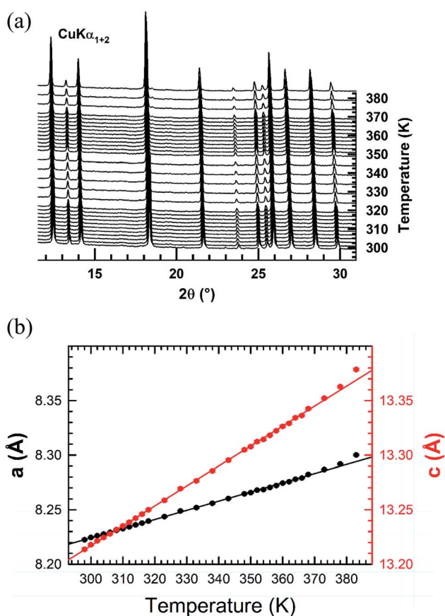
Fig. 5 (a) XRPD patterns collected upon heating in air from RT to 383 K after in situ dehydrating the [(C_2H_5)_4N]FeCl_4 compound at 373 K. (b) Thermal evolutions of the hexagonal cell parameters a and c of the [(C_2H_5)_4N]FeCl_4 compound determined from the refinement of the XRPD patterns by the Le Bail method.
