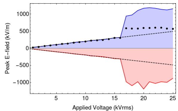
Fig. 5. Peak E -field induced as a function of the applied voltage. Blue: positive peak values. Red: negative peak values. Dashed lines linked to the fitting curves of the linear zone before the threshold. Black dots represent the amplitude of the radial electric field at 50 Hz as a function of the applied voltage.
