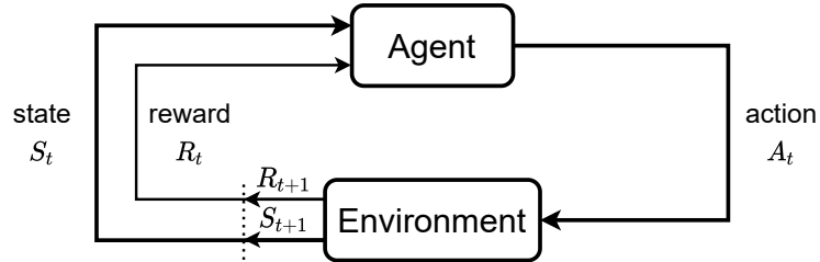
Figure 6: Reinforcement learning.
