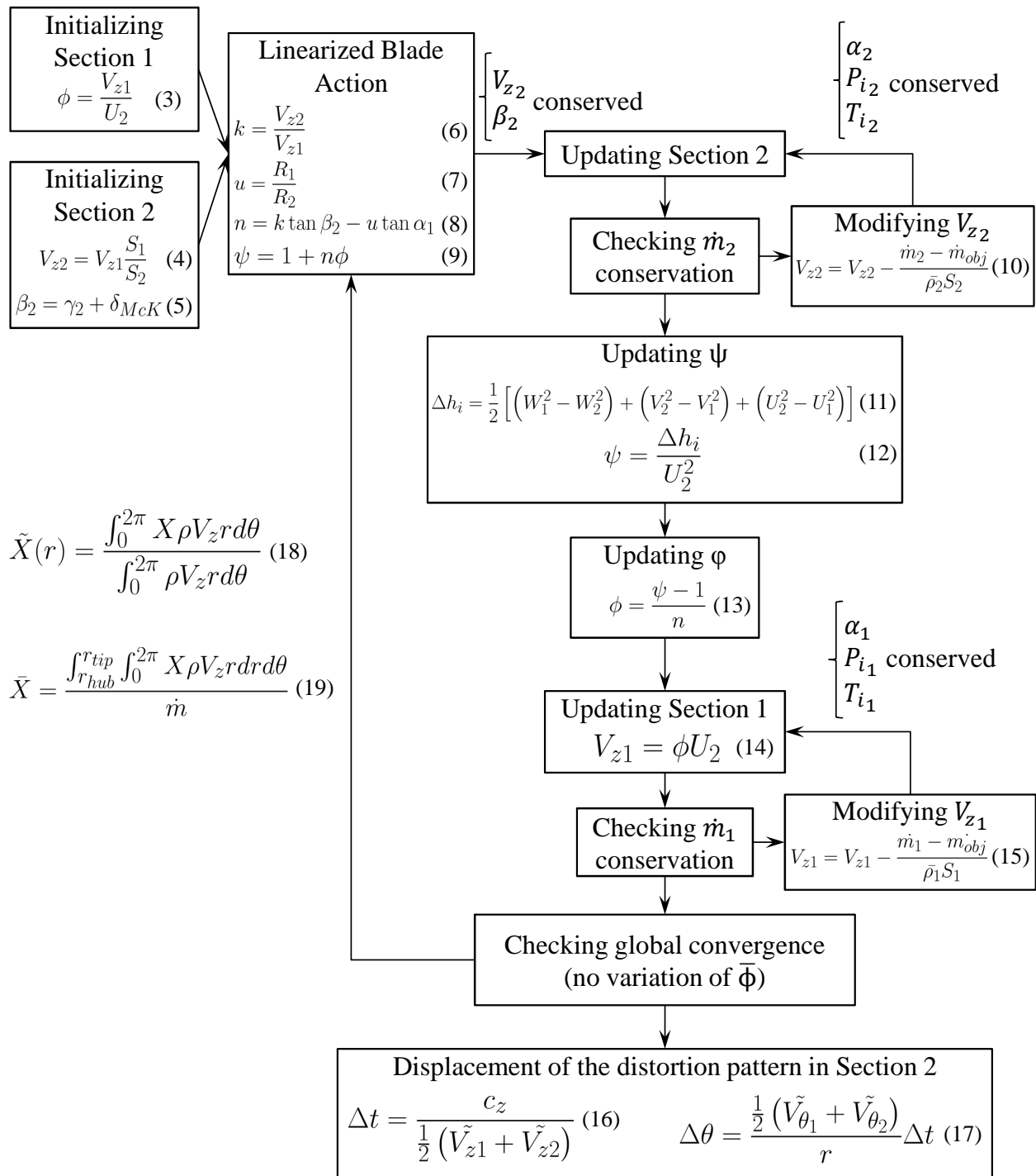
Figure 5. Local parallel compressor workflow.
