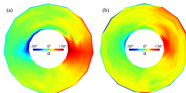
Figure 10. Swirl angle measured at rotor LE: compressor (a) and free windmill (b).
