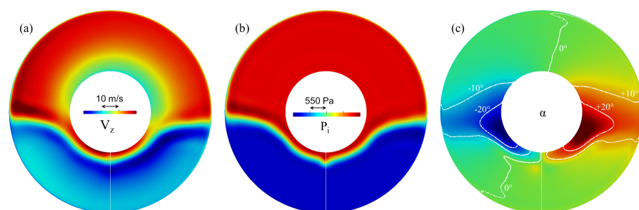
Figure 8. (a–c) Boundary conditions used in PC model for the compressor operating point ( T_i is uniform).
