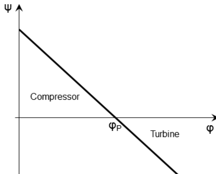
Figure 1. Performance curve plotted in the \phi - \psi framework.
