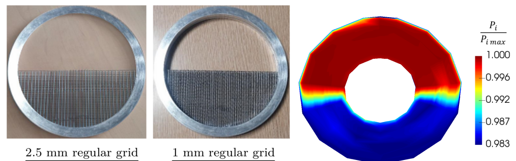
Figure 7. Distortion grids and example of measured total pressure pattern.
