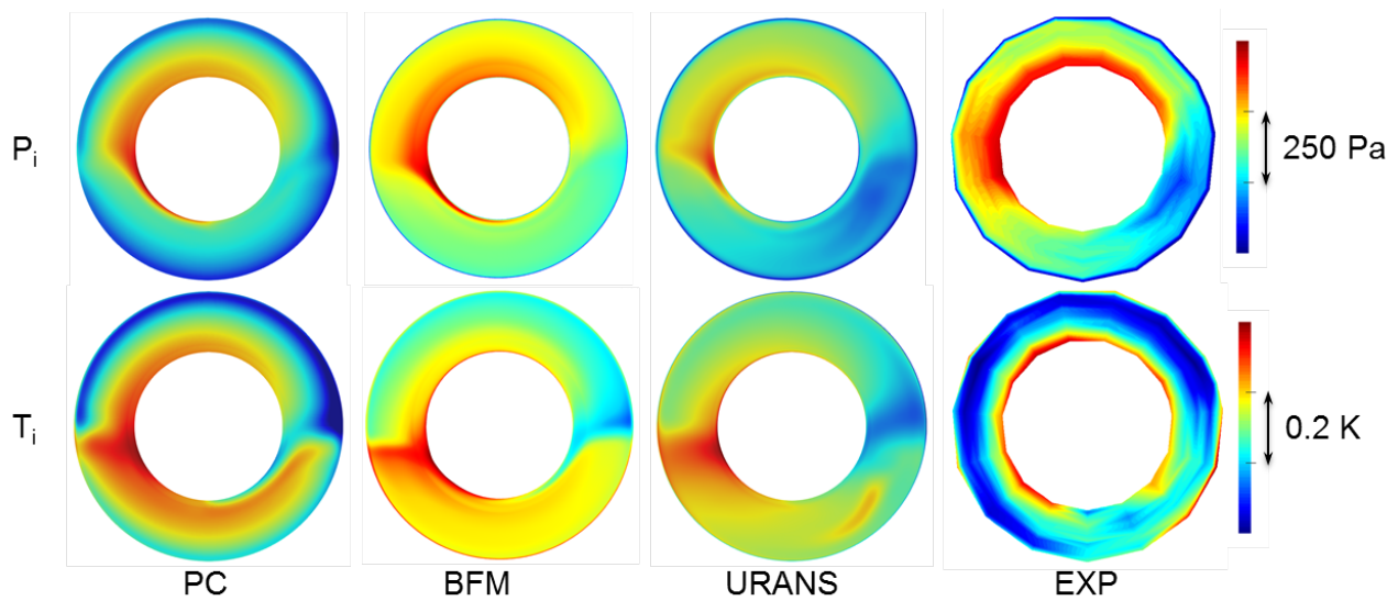
Figure 13. Total pressure (top) and total temperature (bottom) downstream of the rotor.
