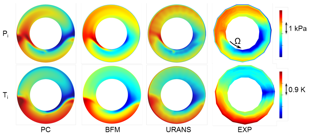
Figure 11. Total pressure (top) and total temperature (bottom) downstream of the rotor.
