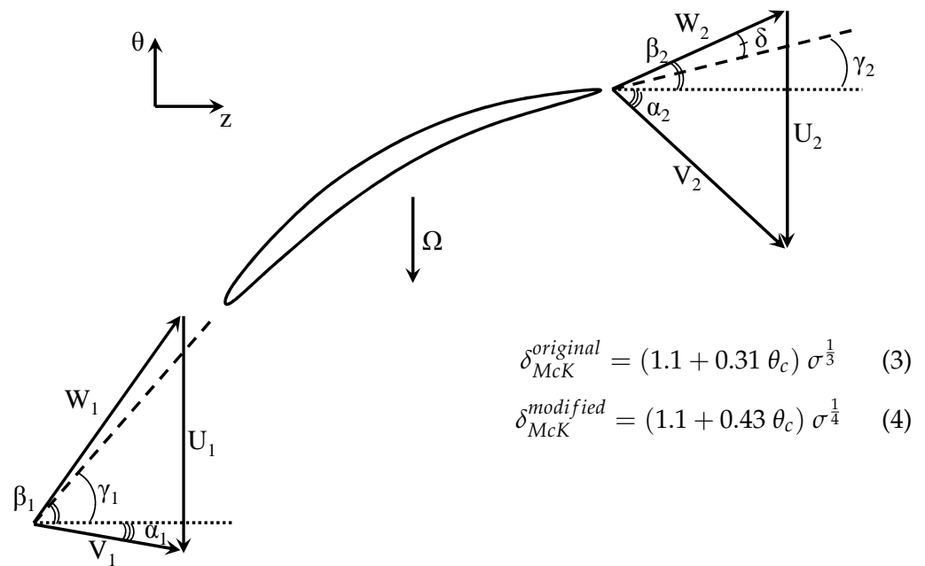
Figure 3. Velocity triangles upstream and downstream of the rotor row.
