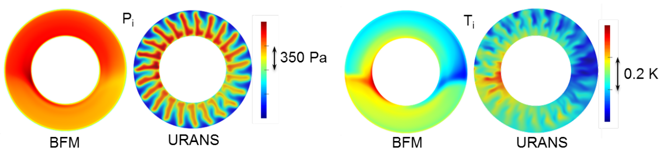
Figure 14. Total pressure (left) and total temperature (right) downstream of the stator.
