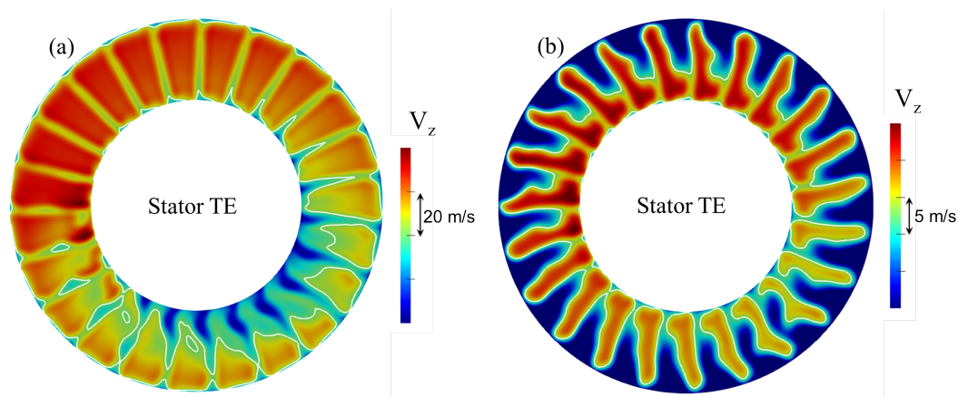
Figure 15. Axial velocity downstream of the stator: compressor (a) and free windmill (b).
