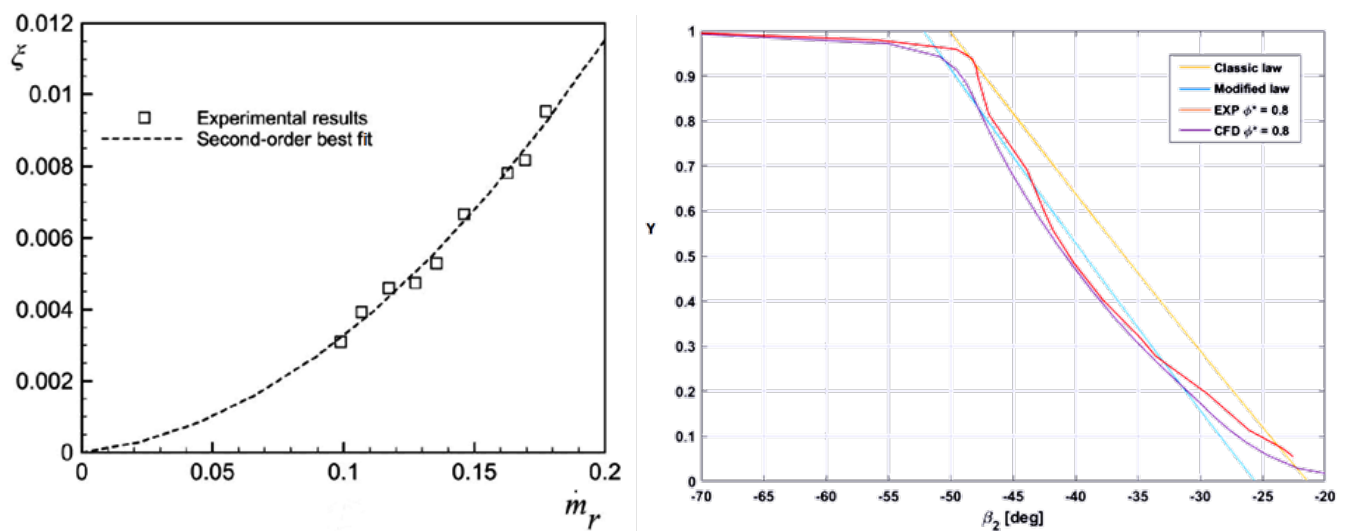
Figure 2. Loss correlation (left) and modified MacKenzie's law at rotor TE (right).
