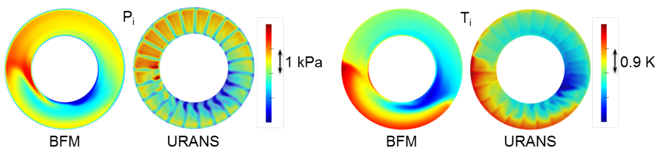
Figure 12. Total pressure (left) and total temperature (right) downstream of the stator.
