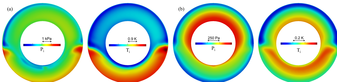
Figure 16. Total pressure and total temperature downstream of the rotor, assuming the same V_z , P_i , T_i conditions from URANS and uniform zero swirl angle: compressor (a) and free windmill (b).
