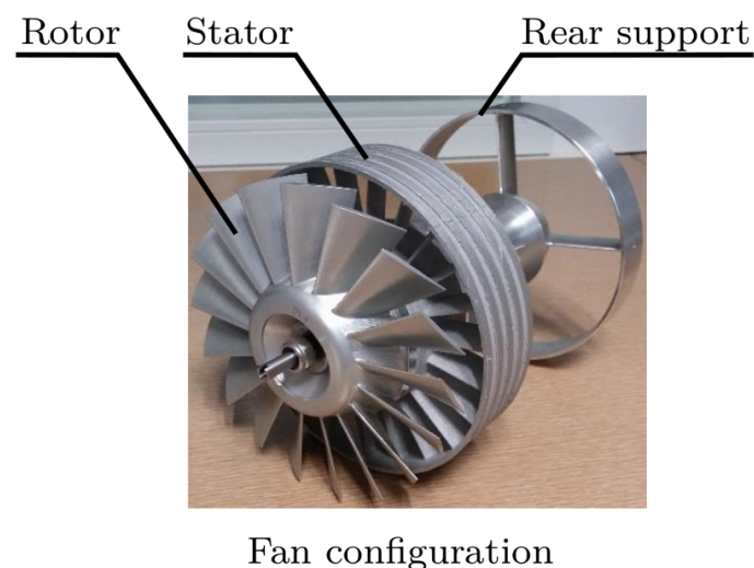
Figure 6. 3D view of the fan stage.
