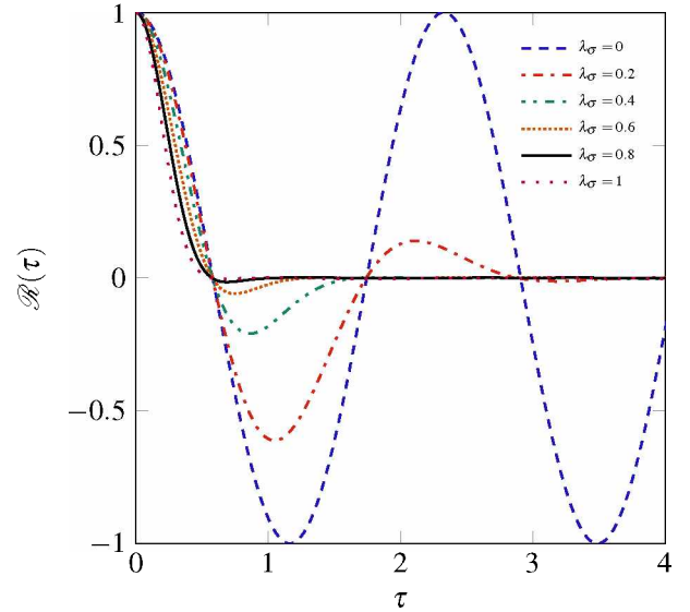
FIG. 2: Two-time correlation functions of the synthetic velocity u_i^s for different Gaussian distributions \lambda \sim \mathcal{N}(\lambda_m = 0.6, \lambda_\sigma) . Calculated from Eq 16.
