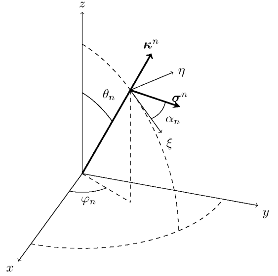
FIG. 1: Wave vector geometry of the n^{\text{th}} Fourier mode.
