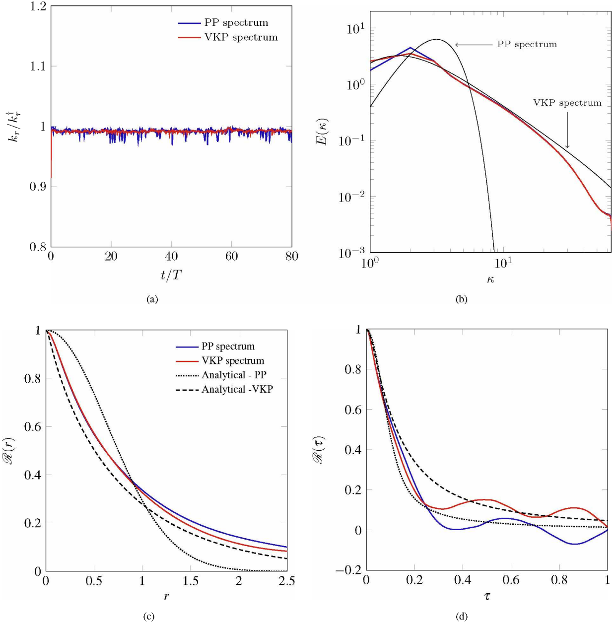
FIG. 10: Comparison between a prescribed PP and VKP spectrum for selective forcing at low wave numbers with a stochastic straining frequency. (a) Time evolution of the kinetic energy, (b) energy spectra, (c) two-point correlation functions and (d) two-time correlation functions.
