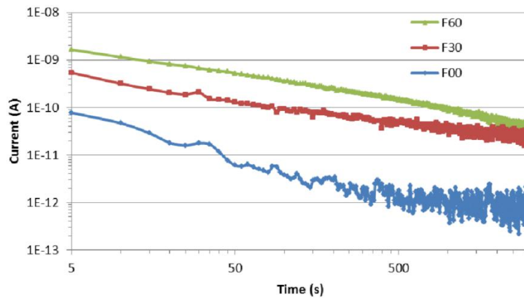
Figure 5. DC conductivity measurement for 250µm epoxy resin sample being treated after different fluorination time [29].
