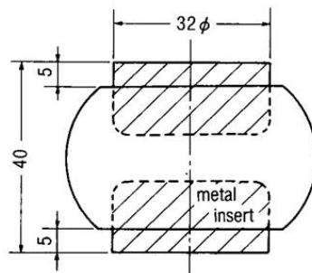
16 17 18 19 20 21 22 23 24 25 26 27 Figure 34. Spacer model designed by Fujinami [56]. 28
