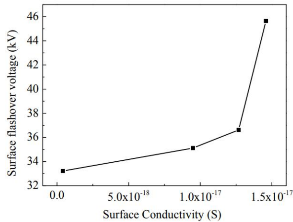
10 11 12 13 14 15 16 17 18 19 20 21 22 23 24 25 26 27 Figure 12. Relation between surface flashover voltage and surface conductivity [44]. 28
