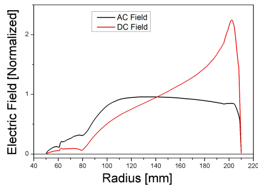
Figure 43. Comparison between capacitive and steady-state resistive electric field strength distribution (gas side) for the HVAC partition [101].
