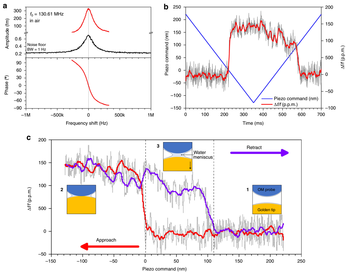
Fig. 6 Approach–retract experiment in air. a Characterization of the optomechanical probe. Black line: noise spectral density showing the Brownian motion of the device (resolution bandwidth = 1 Hz). The resonance frequency is f_0 = 130.61 MHz, Q = 870 in air. The vibration amplitude indicated in the y-axis of the chart is calibrated from the Brownian motion considering an effective mechanical stiffness of 40 kN/m (see “Methods”). The measurement noise floor is below 3 \times 10^{-16} m/ \sqrt{\text{Hz}} . Red line: frequency response in magnitude and phase of the device driven optically (measurement bandwidth: 1 kHz). The measurement background is canceled by the subtraction of a vector signal at the driving frequency. The vibration amplitude is 0.32 pm at resonance. b Blue line: command applied to the Z piezo actuator versus time during the approach–retract experiment. Red line: relative shift of the resonance frequency of the optomechanical probe (see “Methods”). The measurement raw data are plotted in gray (acquisition rate: 1 MSa/s). The red line results from a moving average. The probe is actuated at resonance with a free vibration amplitude of 0.32 pm. c Variation of the relative shift of the mechanical resonance frequency versus the Z piezo actuator command. Red line: approach of the sample toward the optomechanical probe (the distance to contact is reduced). Purple line: retract from the optomechanical probe. The measurement raw data are plotted in gray (acquisition rate: 1 MSa/s). Colored lines result from a moving average. The probe is driven at the resonance frequency with a free vibration amplitude of 0.32 pm. Insets 1–3: schematic of the interaction between the optomechanical probe and the golden tip sample showing the formation of a water meniscus responsible for the hysteresis in the force curve.
