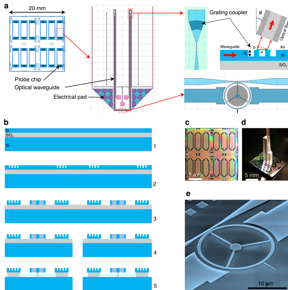
Fig. 3 Design and fabrication of the optomechanical probe. a 2 cm × 2 cm unit cells are repeated on 200 mm wafers, each containing 12 probe chips. The optomechanical ring resonator holding the AFM tip is placed at the edge of the probe chip, surrounded by large pads for electrical interconnects to the capacitive electrodes. The optical waveguide extends up to the center of the probe chip. Its ends are connected to grating couplers patterned in the silicon device layer. The geometrical parameters (period a , height d_g ) define the first-order diffraction angular direction \theta , allowing the guided light to be coupled out of plane to optical fibers. b Overview of the main steps of the fabrication process. 1—Photonic-grade silicon-on-insulator (SOI) wafers for fabrication. The device layer, buried oxide layer, and handle layer thicknesses are 220 nm, 1 \mu m, and 725 \mu m, respectively. 2—Lithography and partial plasma etching of the device layer (etching depth = d_g ) for the realization of diffraction gratings. 3—Variable shape electron beam lithography and plasma etching of the device layer for the realization of all parts of the optomechanical probes. 4—Dicing of individual probe chips. 5—Releasing step by time-controlled etching of the buried oxide layer in vapor HF. c Optical microscopic image of a unit cell containing 12 devices at step 3 of the fabrication process. d View of a device with a glued transposer allowing interconnections between the grating couplers and the optical fibers. e Scanning electron microscopic image of a fabricated optomechanical probe. The ring diameter and width are 20 \mu m and 750 nm, respectively. The 3 spokes are 500 nm wide. The tip length is 5 \mu m. The gap distance between the waveguide and the ring is g = 100 nm. The distance between the capacitive transducers and the ring is 1 \mu m.
