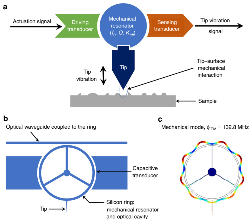
Fig. 2 Introduction of the AFM probe with optomechanical transduction. a Block diagram of the principle of operation of an AFM probe in dynamic mode. b Schematic of the optomechanical AFM probe (top view). The silicon ring is the mechanical resonator of the AFM probe, which supports high quality factor optical modes coupled to mechanical modes. The ring is anchored by three spokes. A waveguide is evanescently coupled to the optical ring cavity, enabling optomechanical transduction readout. The probe tip is diametrically opposed to the evanescent coupling region. c Calculation by finite element modeling (FEM) of the modulus of the displacement of the mechanical mode under study in this work. A resonance frequency of f_{FEM} = 132.8 MHz is obtained here for a ring 20\ \mu\text{m} in diameter and 220\ \text{nm} in thickness, corresponding to our design parameters.
