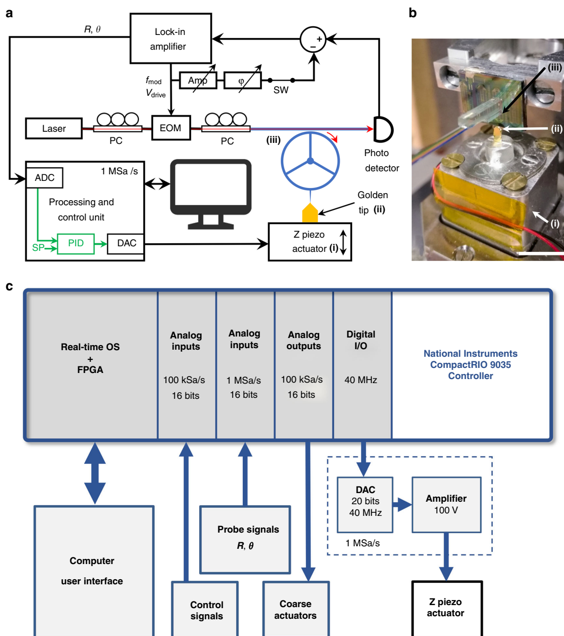
Fig. 5 Instrument set-up for approach–retract experiments and closed-loop operation. a Block diagram of the custom scanning-probe instrument used for the experiments in an AFM configuration. The optomechanical probe is optically actuated and detected. An extra signal path allows the generation of a vector signal derived from the driving signal at frequency f_{\text{mod}} . This vector signal is tunable in amplitude (Amp) and phase ( \varphi ) and is subtracted from the probe signal before demodulation by the fast lock-in amplifier (LIA). The demodulated information is then fed to the control unit, which processes 10^6 samples per second. The unit contains a proportional-integral-derivative controller (PID) and drives the Z piezo-actuator (i), which sets the distance between the golden tip used as the sample (ii) and the optomechanical probe (iii). PC phase controller, EOM electro-optical modulator, SW switch, ADC analog-to-digital converter, DAC digital-to-analog converter, SP setpoint. b Close view (optical image) of the AFM head, scale bar: 10 mm. The displacement range of the Z piezo actuator (i) is 2 \mu\text{m} , and its displacement bandwidth is 100 kHz. The mobile flange of the actuator holds sample (ii), which is a golden tip. A piezo stage located below the Z piezo actuator is used to set the position of the sample along the XY directions. The AFM optomechanical probe (iii) is placed vertically, and its tip apex points toward the sample. The optical fibers are glued to the probe chip by means of a transposer aligned with the grating couplers. c Details of the processing and control unit implemented on a National Instruments CompactRIO 9035 controller, featured with an FPGA (field-programmable gate array), a real-time processor, and an embedded user interface capability. All parts of the system are programmed with the LabVIEW software. Several input/output modules allow the acquisition/generation of signals. A 20-bit DAC and a high-voltage amplifier were specifically designed for the application, offering the resolution and speed required to drive the Z piezo actuator. Extra input/output signals are available for the purpose of controlling the instrument. This includes the displacement of the XY piezo stage up to 10 frames/s.
