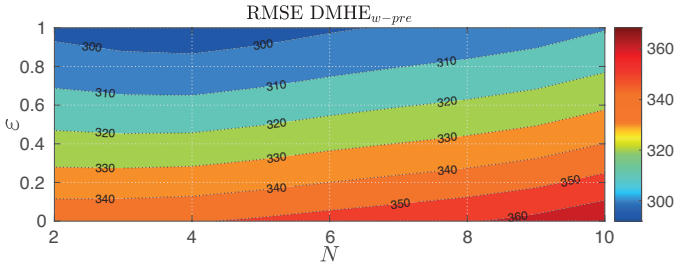
Fig. 5: Sum of x_0 -averaged RMSEs of the proposed \text{DMHE}_{w\text{-pre}} with K varying as in (23).
