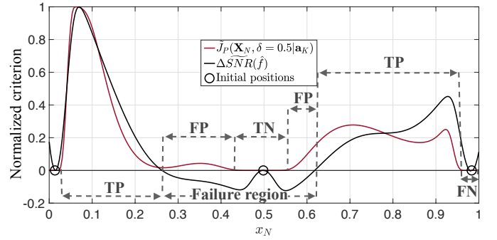
Fig. 4: Region classification: Positive ( P ) vs. Negative ( N ), and True ( T ) vs. False ( F ). P and N represent the regions where \widetilde{\Delta SNR}(\hat{\mathbf{f}}) is positive and negative, respectively. T is a situation when the criterion and \widetilde{\Delta SNR}(\hat{\mathbf{f}}) are both positive, or the criterion is zero and \widetilde{\Delta SNR}(\hat{\mathbf{f}}) is negative. F is when the criterion is positive while \widetilde{\Delta SNR}(\hat{\mathbf{f}}) is negative, or the criterion is zero whenever \widetilde{\Delta SNR}(\hat{\mathbf{f}}) is positive.
