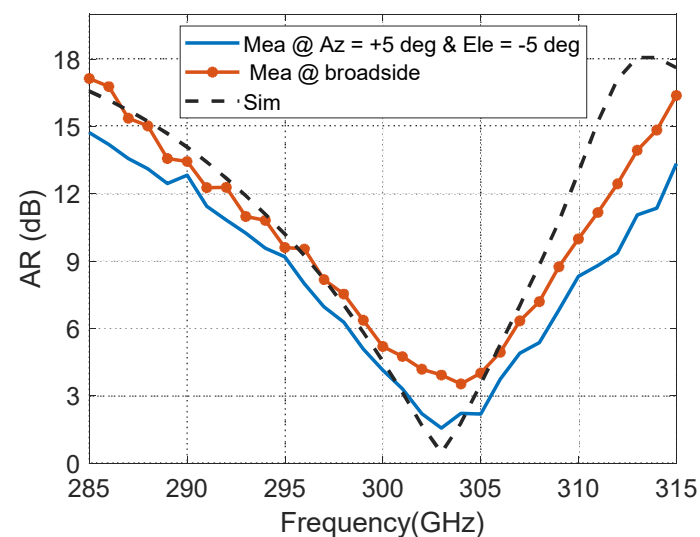
Figure 6. Measured and simulated axial ratio (AR) of the proposed antenna.
