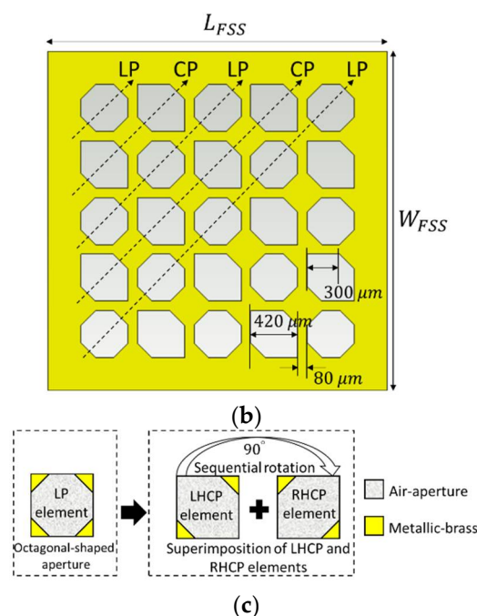
Figure 1. 300 GHz CP-RCA: (a) exploded model view of 7-layered-structures (brass used for all layers) [25]; (b) top view of metasurface layer (dimensions is inset); and (c) graphical demonstration of the working principle of the proposed LP octagonal-shaped aperture.
