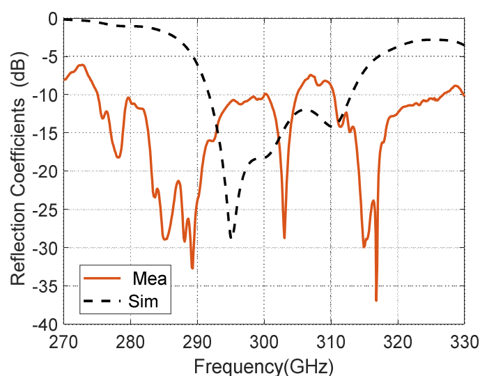
Figure 3. Measured and simulated of the reflection coefficients (S11) of the CP-RCA.
