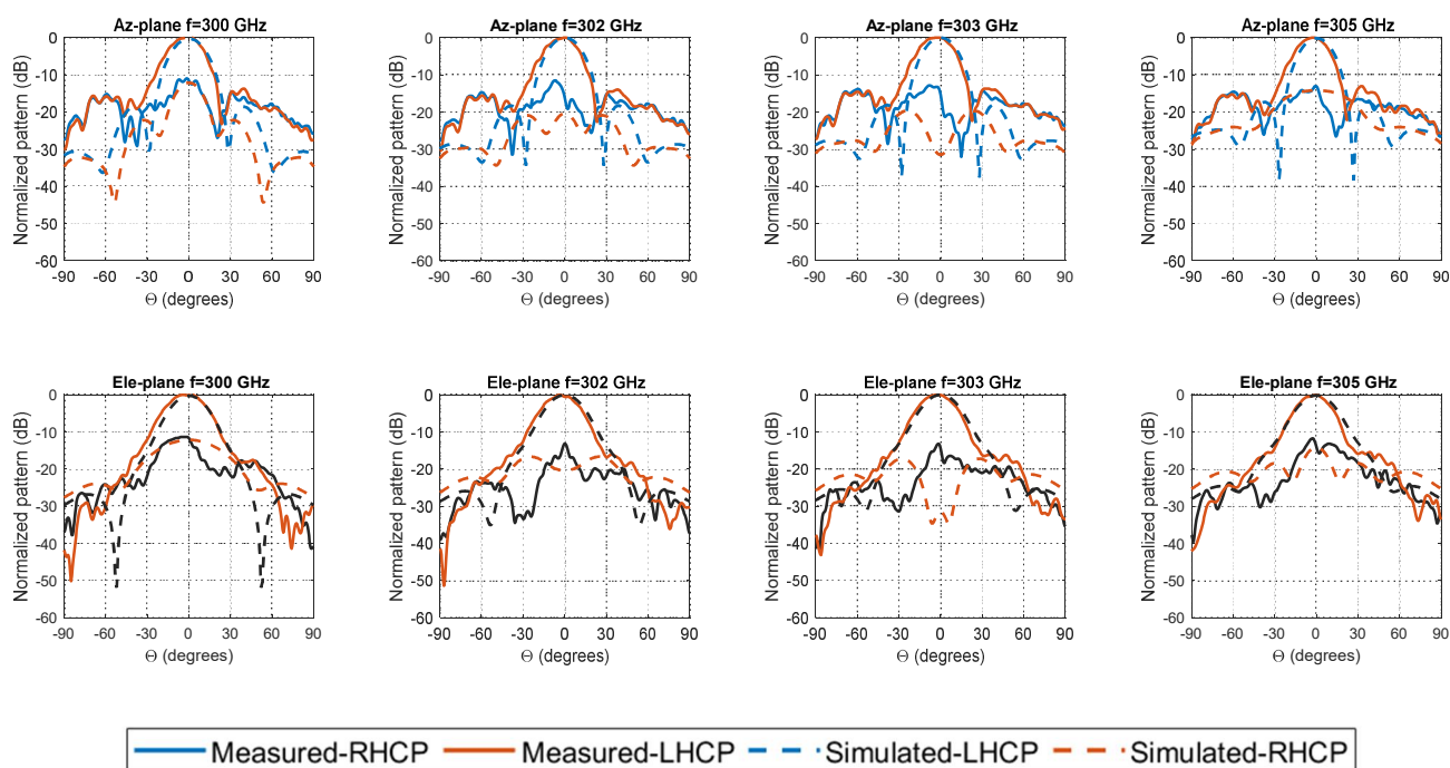
Figure 8. Measured (solid lines) and simulated (dashed lines) radiation pattern of the CP-FPC antenna at 300, 302, 303, and 305 GHz for azimuth (Az.), and elevation (Ele.)-plane cuts.
