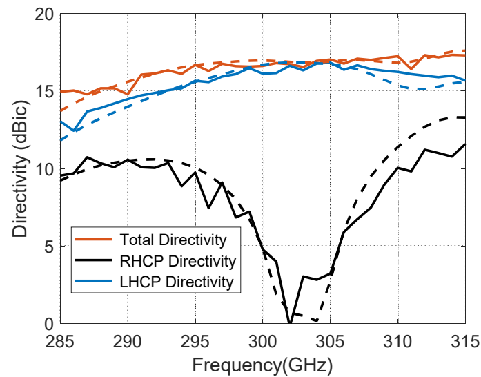
Figure 5. The measured (solid lines) and simulated (dashed lines) of the total, LHCP, and RHCP directivities for the proposed antenna.
