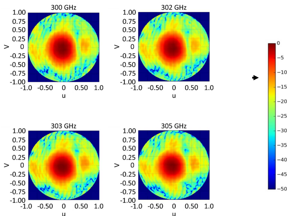
Figure 9. Measured LHCP components of the directivity for the CP-RCA antenna in the u - v spectral plane at different frequencies. The color bar is on the dB scale.
