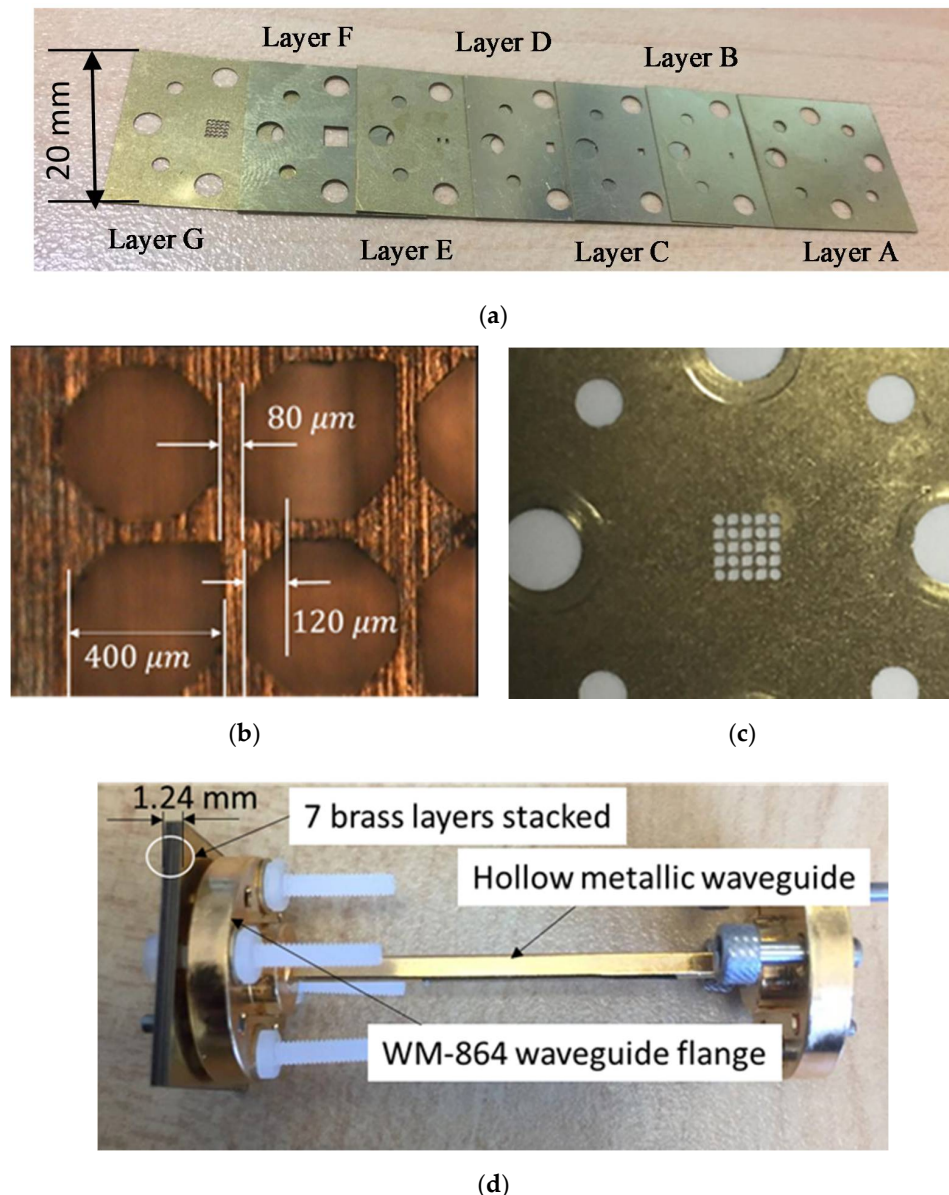
Figure 2. Photographs of manufactured CP-RCA at 300 GHz (a) seven metal brass fabricated layers; (b) microscopic image of MTS layer; (c) enlarged image of CP-MTS layer; and (d) fabricated prototype connected to standard UG–387/U waveguide flange [25].
