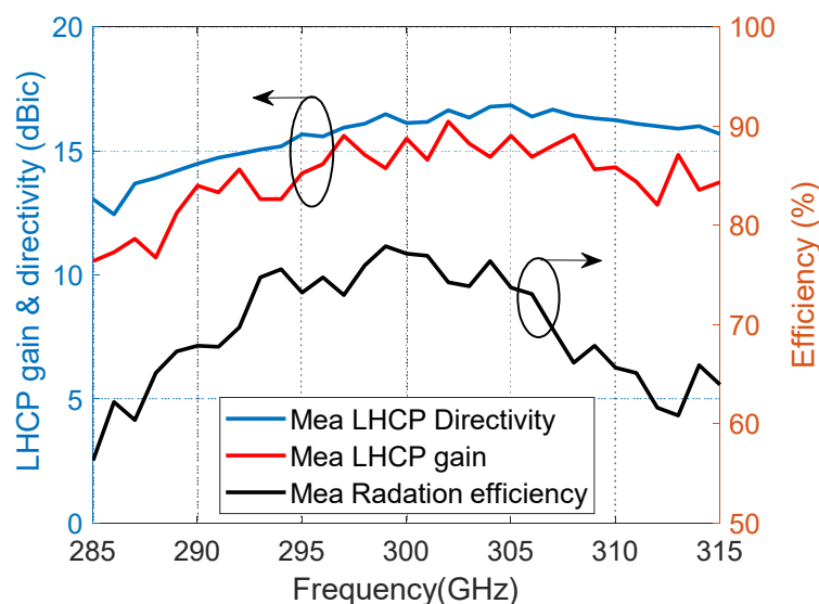
Figure 4. Measured LHCP directivity, realized gain, and radiation efficiency of the proposed antenna.
