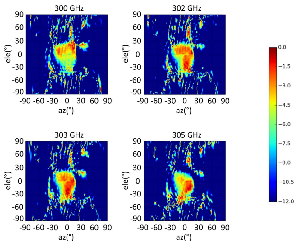
Figure 7. Measured 2D AR of the proposed antenna at different frequencies.
