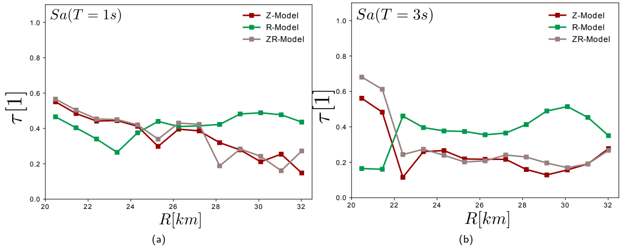
Figure 17: Standard deviation \tau of the between-event residual \delta B_e computed along source-to-site distance R , for T = 1 s (a) and T = 3 s (b).
