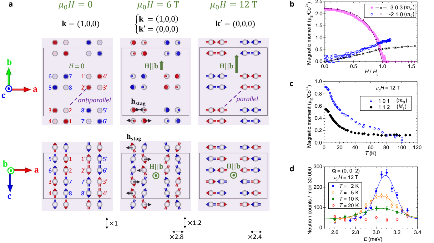
FIG. 2. Static properties in a transverse magnetic field. a , Magnetic structures of \text{BaCo}_2\text{V}_2\text{O}_8 in a uniform field \mathbf{H} \parallel \mathbf{b} shown in the (\mathbf{a}, \mathbf{b}) plane (top) and in the (\mathbf{a}, \mathbf{c}) plane (bottom) at 0, 6, and 12 T, obtained from neutron diffraction experiments performed on the D23 diffractometer. The two kinds of chains are plotted in red and blue, respectively, and the Co atoms are numbered in the zero-field panels, like in Ref. 3 . For a better visualization, the amplitude of the magnetic moments was multiplied along the \mathbf{a} and \mathbf{c} axes by the values indicated below the figures. The staggered field \mathbf{h}_{\text{stag}} is represented with black arrows, only in the panels corresponding to the 6 T magnetic structure for one chain. The end collinear magnetic structures have different propagation vectors, \mathbf{k} and \mathbf{k}' indicated above the figures, and thus have different interchain magnetic arrangements: For H = 0 , the bonds along \mathbf{a} \pm \mathbf{b} are AF aligned while they are ferromagnetically (FM) aligned for \mu_0 H = 12 \text{ T} (see dashed purple line). Consequently, the contributions to the total energy of bonds along \mathbf{a} and \mathbf{b} cancel each other for H = 0 , half of them being frustrated, at variance with the non frustrated 12 T structure in which the bonds along \mathbf{a} and \mathbf{b} are both AF aligned. The intermediate magnetic structure, at \mu_0 H = 6 \text{ T} , is described by both propagation vectors \mathbf{k} and \mathbf{k}' , and is thus non collinear. b , Field dependence of the staggered magnetic moments of the two competing magnetic phases determined at 1.5 K from the square root of the intensity of the \bar{2}01 and 303 pure magnetic reflections for the low and high field phases respectively (pink and blue circles). These experimental staggered moments m_c and m_a are compared to the ones calculated by numerical simulations (red and blue crosses connected by solid lines). c , Temperature dependence at \mu_0 H = 12 \text{ T} of the AF ( m_a ) and FM ( M_{\parallel} ) components of the high field phase, obtained from the square root of the intensity of the 101 and 112 reflections, respectively. d , Temperature dependence of the lowest energy magnetic excitation at a zone center position and at \mu_0 H = 12 \text{ T} , measured on the IN12 three-axis spectrometer. The solid lines are Gaussian fits.
