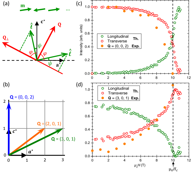
FIG. S2. (a) Rotating local frame ( \hat{\ell} , \hat{\mathbf{b}} , \hat{\mathbf{t}} ). The \hat{\ell} (resp. \hat{\mathbf{t}} ) unitary vector is parallel (resp. perpendicular) to the ordered magnetic moment. The directions of the scattering vector \mathbf{Q} and of \hat{\ell} with respect to \mathbf{a}^* are identified by the \varphi and \psi angles, respectively. (b) Location in the reciprocal lattice of the AF and ZC positions investigated. (c, d) Spectral weight of the lowest energy branch as a function of the transverse field for \mathbf{Q} = (0, 0, 2) and \mathbf{Q} = (3, 0, 1) ZC positions respectively, as measured (orange points), and calculated for longitudinal (green circles) and transverse (red circles) fluctuations. This clearly evidences the transverse nature of this excitation mode.
