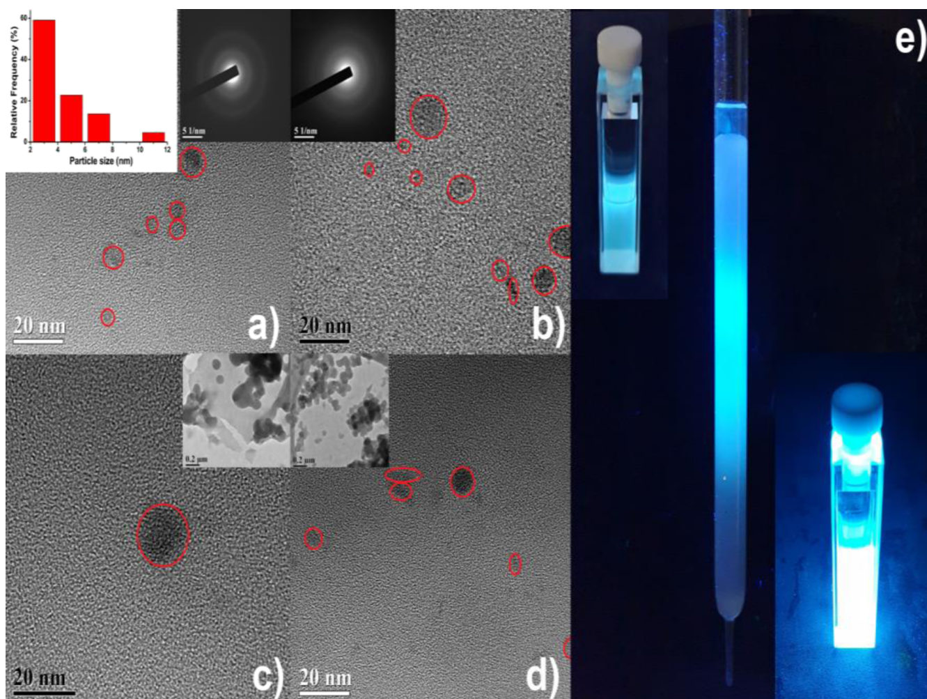
Figure 2. (a–d) TEM images of carbon NPs. Insets in (a,b): SAED patterns and the histogram of particle size distribution from the captured carbon NPs. Insets in (c,d): aggregated carbon NPs. (e) Chromatographic column with carbon NPs and their alcohol solutions under UV excitation, under 365 nm radiation.
