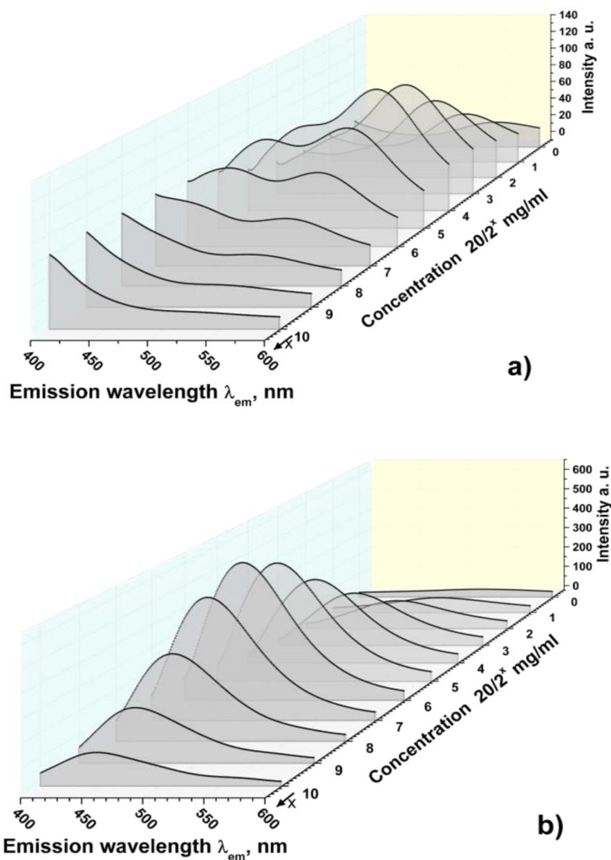
Figure 3. Intensity of emission spectra recorded at (a) \lambda_{\text{ex}}^1 = 285 \text{ nm} and (b) \lambda_{\text{ex}}^2 = 355 \text{ nm} against the concentration of carbon NPs.
