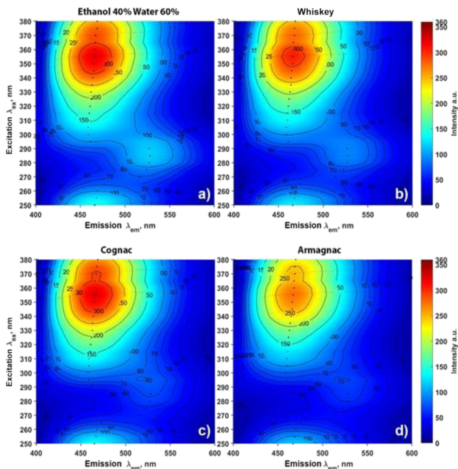
Figure 4. PL maps for the solution of carbon NPs ( c_{\text{NP}}^4 = 20/2^4 mg/mL) in the presence of analyte: (a) ethanol/water solution (40/60 vol), (b) whiskey, (c) cognac, and (d) armagnac.
