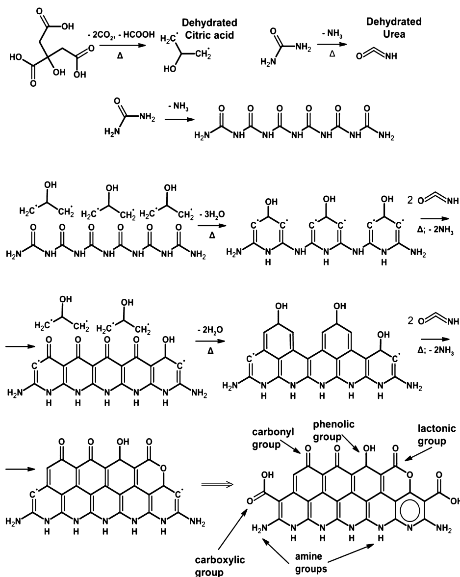
Figure 1. Possible thermochemical transformations producing carbon NPs. Growth mechanism of carbon NPs with increasing temperature and growth time.
