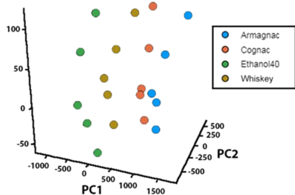
Figure 5. PCA visualization of the components from the analysis of PL map as the response of sensor system with carbon NPs on the presence of analytes: armagnac, cognac, whiskey, and ethanol/water (40%/60%) mixture.
