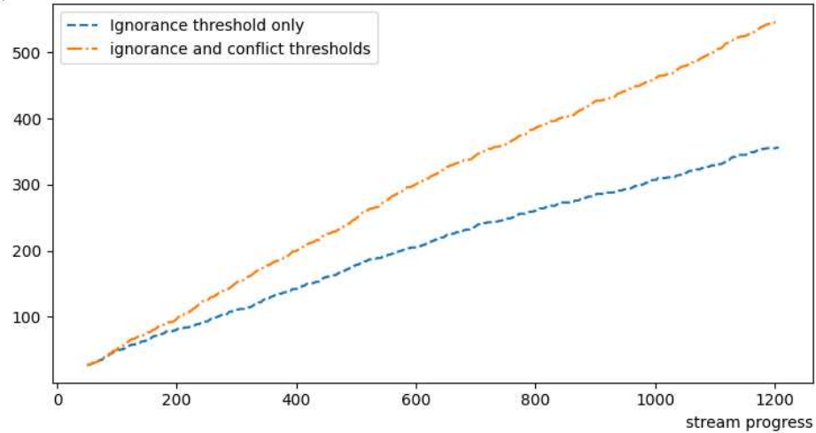
FIGURE 12: Growth of the example database with the progress of the stream for two AL models.
