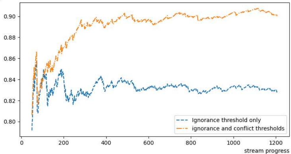
FIGURE 13: Evolution of AAS^{pre\text{ }pro} with the progress of the stream for two AL models.
