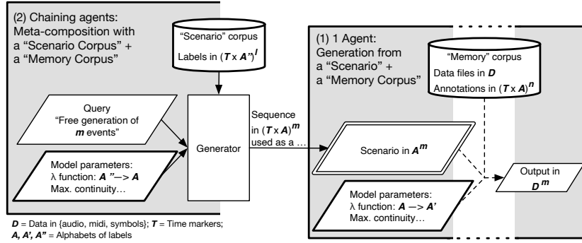
Fig. 4. Navigation through a “Memory Corpus” guided by (1) explicit scenarios manually inputted or (2) scenarios generated by another agent.
