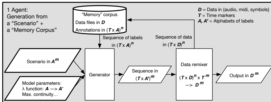
Fig. 1. Architecture of a DYCI2 generative agent.
