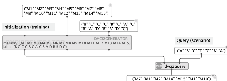
Fig. 2. A simple OM-DYCI2 process in OM#. Left: Initializing a DYCI2-GENERATOR from a memory defined by a list of contents such as MIDI data, time markers in an audio file, etc. (M1, M2, ...) and a corresponding list of labels (A, B, C, D). Right: Querying the DYCI2-GENERATOR with a scenario. Dataflow is top-down, triggered by evaluation requests at the bottom of the patch.
