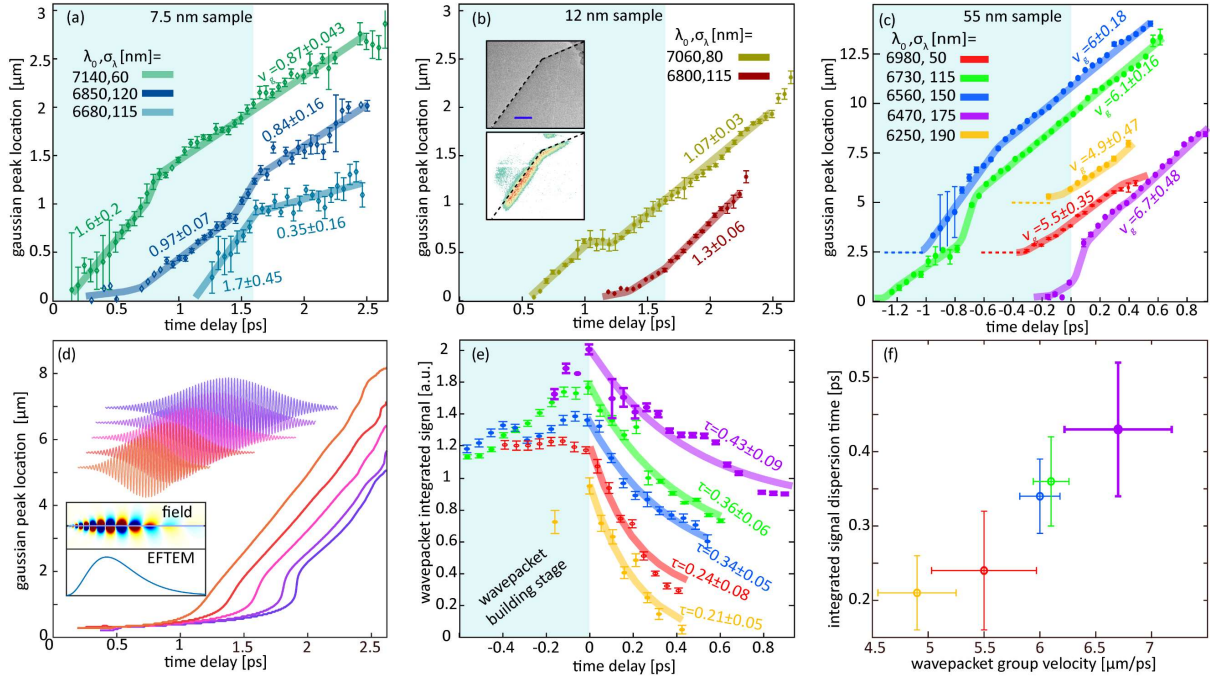
Fig. 3. Analysis of the PhP wavepacket formation, propagation, and decay - extracting the group velocities and wavepacket behavior. (a-c) The fitted Gaussian peak locations as a function of time with the extracted group velocities in units of \mu\text{m}/\text{ps} . We compare three \text{h}^{11}\text{BN} samples having a thickness of (a) 7.5 nm, (b) 12 nm, and (c) 55 nm. The colored background represents the times at which the wavepacket is still being pumped. For clarity, the measurements are shifted in time from one another; also, the dashed horizontal lines in (c) represents that the blue and red curves are shifted in space by 2.5 \mu\text{m} and the yellow curve by 5 \mu\text{m} . Top inset in (b): unfiltered image of the 12 nm sample (dashed lines represent sample edges); scale bar is 5 \mu\text{m} . Bottom inset in (b): an electron energy loss filtered image showing the group at a specific time. (d) Simulation results of the wavepacket peak location as a function of time in a 55 nm \text{h}^{11}\text{BN} sample, comparing different levels of chirp (the excitations' temporal profiles are brought above the curves). The simulations show the acceleration and deceleration observed experimentally. Top inset: the simulated field. Bottom inset: the energy-filtered electron signal calculated using the field from the top inset, showing that the PINEM technique indeed extracts the wavepacket profile. Further simulations of the velocity change can be seen in Fig. S5 and movies S3 and S4. (e) Wavepacket integrated signal (derivation in the SM section S.3), which helps identify the transition from a formation stage, in which the pump overcomes the dispersion and intrinsic PhP losses, to the eventual decay (the effective timescales are denoted in ps). (f) There is a clear correlation between the dispersion rate and the wavepacket's group velocity, as expected by theory: wavepackets with higher group velocities are less dispersive.
