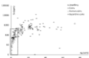
Figure 4 –The amounts of Ag and Sn (references in the text) contained in Visigothic gold jewellery and coins compared to Roman and Byzantine gold coins (inside the rectangle).
