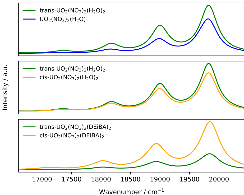
Figure 4: Theoretical vibronic progressions of the \text{UO}_2(\text{NO}_3)_2(\text{H}_2\text{O}) and \text{cis}/\text{trans-UO}_2(\text{NO}_3)_2(\text{L})_2 ( \text{L} = \text{H}_2\text{O} , DEiBA) complexes. The position of the first peak is adjusted to the computed “hot band” value of the \text{trans} -complexes and corrected by the \nu_s of the excited state. The spectral shapes were estimated by convoluting the stick spectra with Lorentzian functions with a FWHM of 400 \text{ cm}^{-1} .
