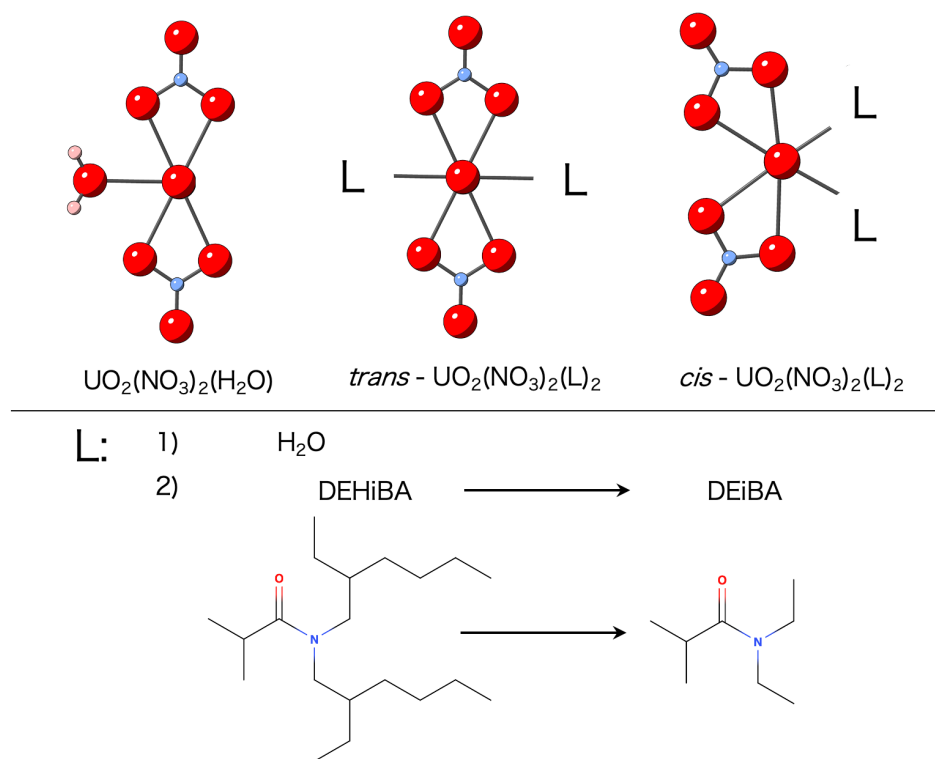
Figure 1: The structures of \text{UO}_2(\text{NO}_3)_2(\text{H}_2\text{O}) and \text{UO}_2(\text{NO}_3)_2(\text{L})_2 ( \text{L} = \text{H}_2\text{O} , \text{DEiBA} ) model systems in their trans - and cis -configurations. The view is made along the z axis defined by the uranyl unit.
