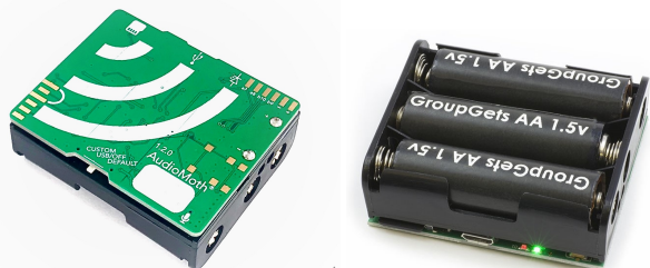
Figure 4: Left: Printed circuit board (PCB) of the AudioMoth sensor. Right: battery holder. Photographs reproduced from the official website of Open Acoustic Devices.
