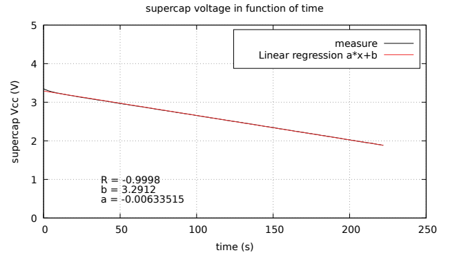
Figure 2: Drop in supply voltage as the FFT is run on the LEA
