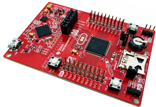
Figure 6: Development kit for the MSP430FR5994 MCU, including embedded FeRAM, a super capacitor, an analog-to-digital converter (ADC), a microSD card slot, and various communication ports.
