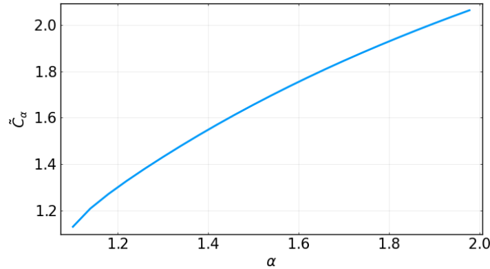
Figure 1: Numerical illustration of the function \alpha \mapsto \tilde{C}_\alpha .
