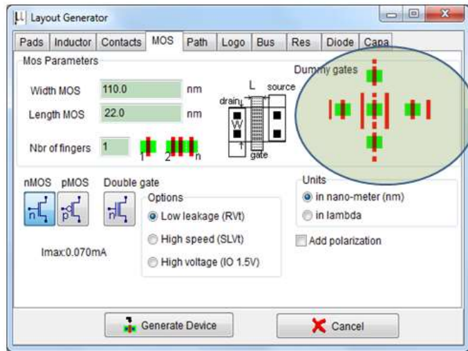
Figure 17: The layout generation includes the dummy gate option at any side (or all sides) of the active MOS device to reduce variability and increase manufacturability
