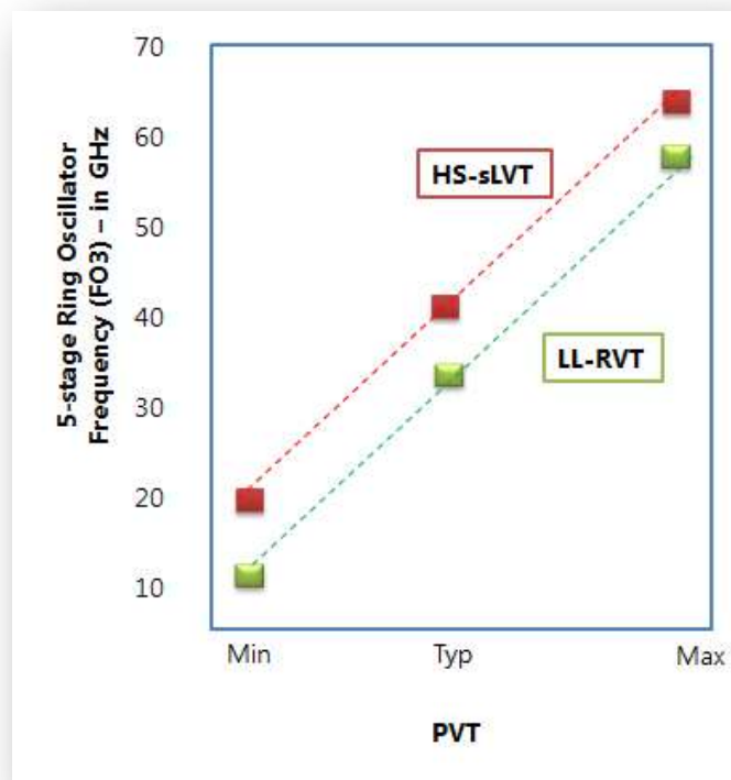
Figure 26: PVT Min-Max simulation showing 300 % variation in oscillating frequency of the ring-oscillator (20nm\RingOsc_5Stage_FO3_Scholze.MSK)
