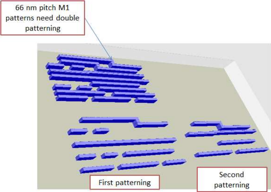
Figure 22: Principles of double patterning (20nm\double-patterning-m1.MSK)
