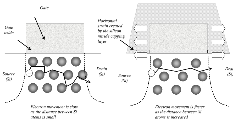
Figure 5: Tensile strain generated by a silicon-nitride capping layer which increases the distance between atoms underneath the gate, which speeds up the electron mobility of n-channel MOS devices
