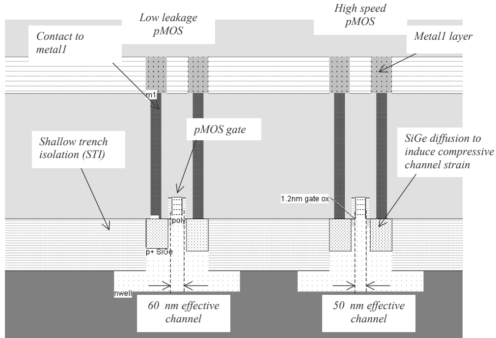
Figure 8: Cross-section of the pMOS devices
