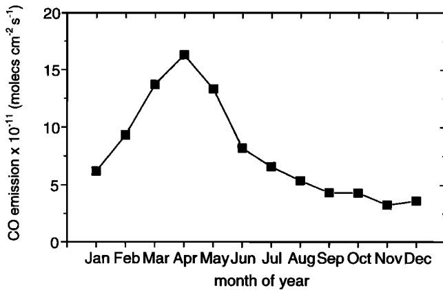
Figure 4. Seasonal variation of mean surface CO flux out of Indochina Peninsula (12.6°–20.9°N, 98.4°–109.7°E) from MOZART 1.
