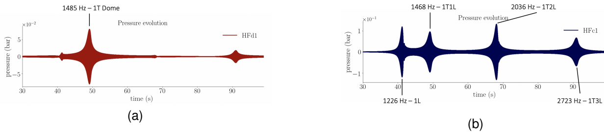
Figure 9: Pressure response in the dome (a) and the chamber (b) from a frequency ramp 0 to 3000 Hz, from StaHF
