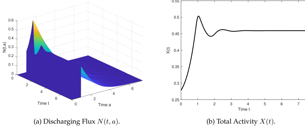
Figure 4: Example 1.1. Case n_0(s, a) = e^{-a} and p = \varphi(X - e^{-s} - e^{-a})\mathbb{1}_{\{s>1\}} .
