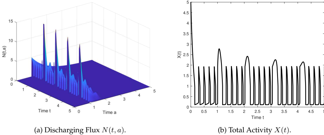
Figure 7: Example 3.1. Case n_0(s, a) = \frac{1}{2}e^{-(a-1)}\mathbb{1}_{\{a > \max(s,1)\}} and p = \varphi(X)\mathbb{1}_{\{s > 1\}} .
