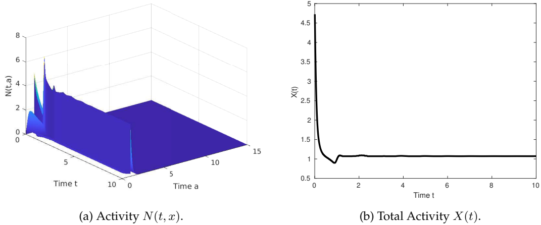
Figure 7: Example 3.2. Case n_0(s, a) = \frac{1}{2} e^{-(a-1)} \mathbb{1}_{\{a > \max(s, 1)\}} and p = \varphi(X) \mathbb{1}_{\{s > 1\}} + \mathbb{1}_{\{s - a > X\}} .
