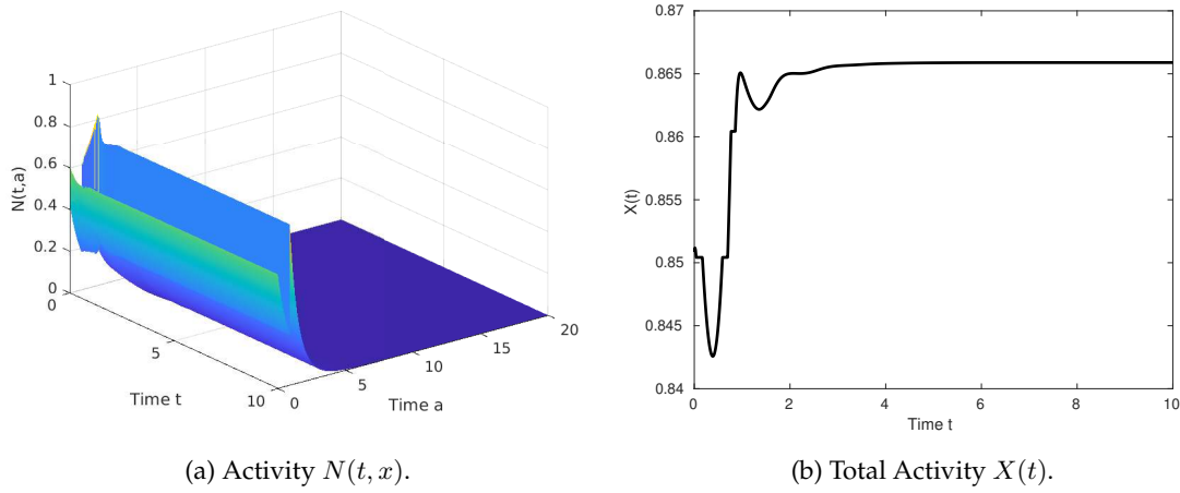
Figure 4: Example 1. Case n_0(s, a) = e^{-a} and p = \mathbb{1}_{\{s > X\}} + \mathbb{1}_{\{s-a > X\}} .
